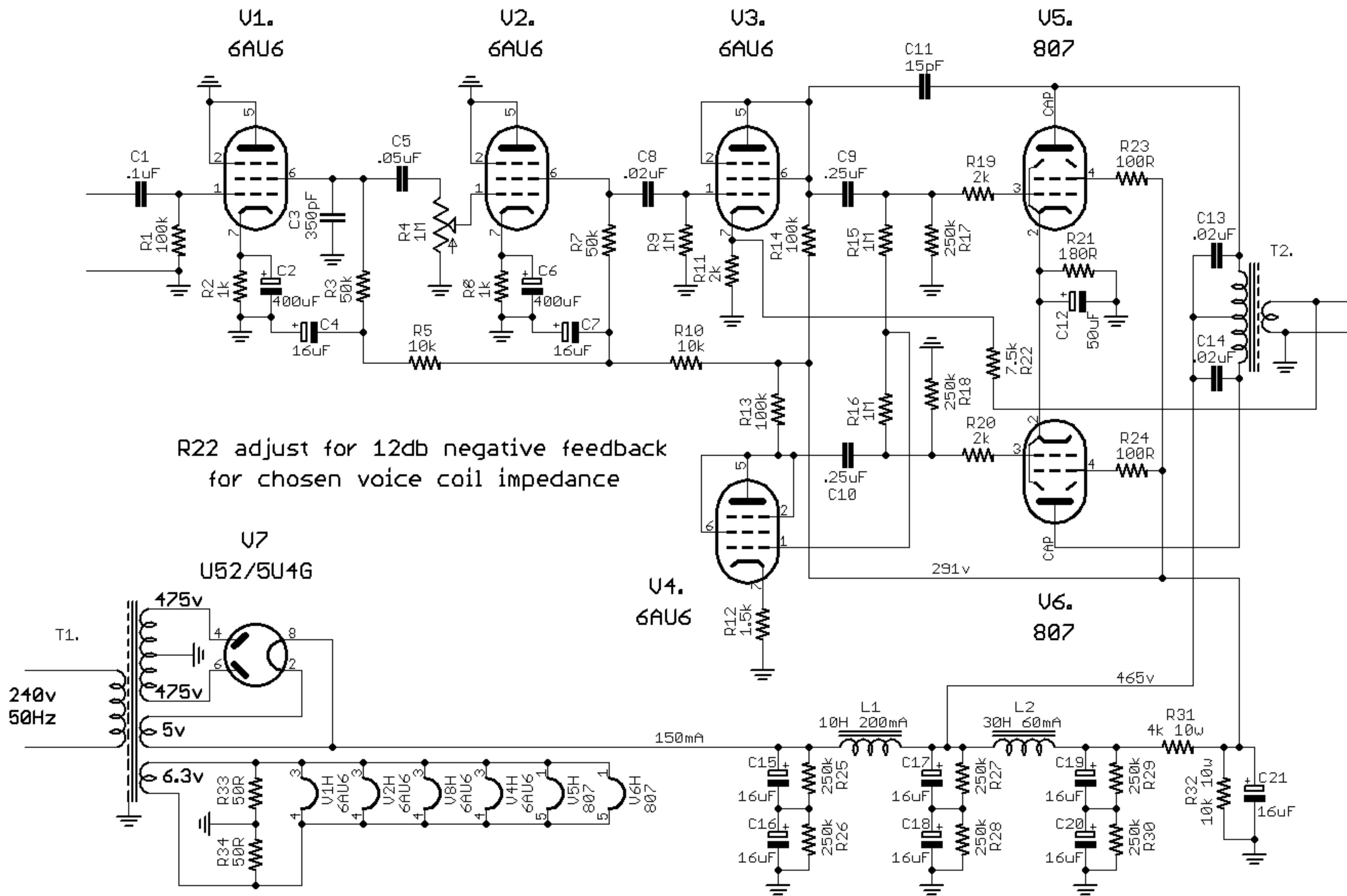
AWV RADIOTRON 25W AMPLIFIER A518 Low Distortion Amplifier using 807 Tetrodes from RADIOTRONICS June, 1950, page 52
