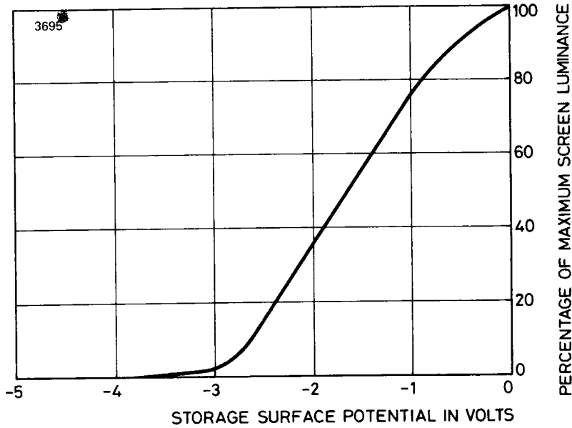
Fig. 3. Typical storage surface potential – screen luminance characteristic
