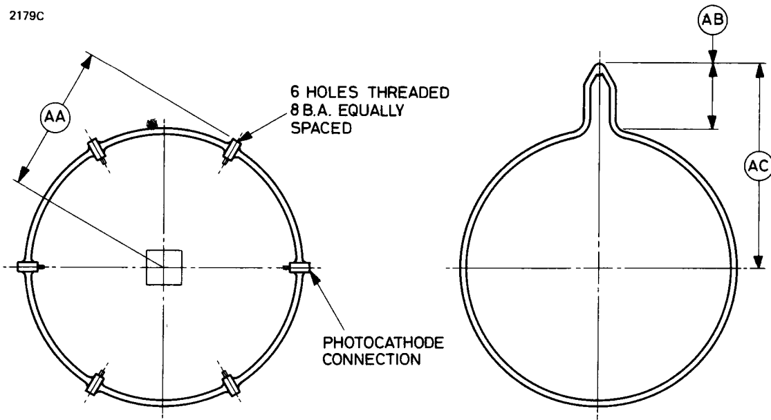
VIEW A-A'
