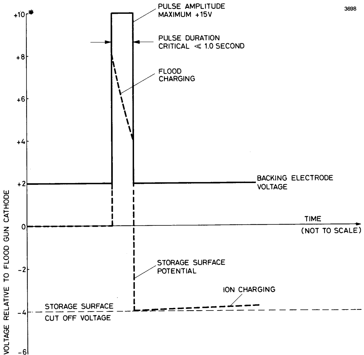
Fig. 6. Short-pulse erase potentials
