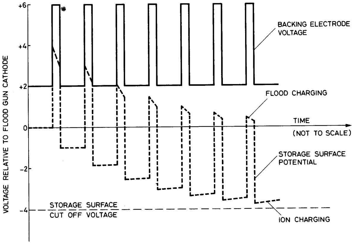
Fig. 7. Pulse train erasure potentials
