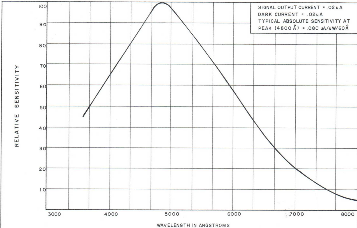
FIG. 4 SPECTRAL RESPONSE
