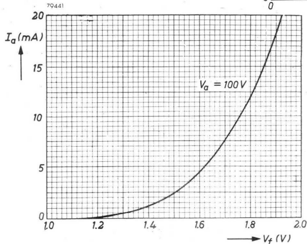
Fig. 66. I_a/V_f characteristic of the K81A at an anode voltage of 100 V.
