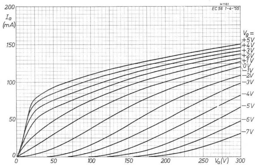
Fig. 43. I_c/V_c characteristics of the EC 56.
