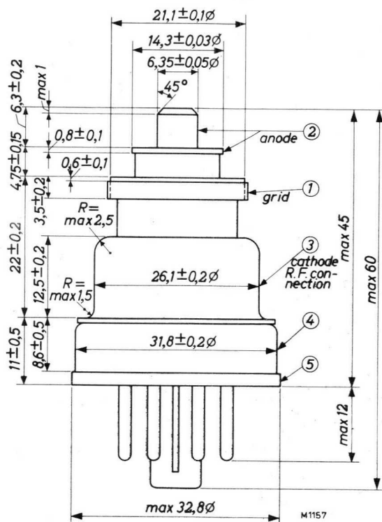
Fig. 39. Dimensional drawing *); dimensions in mm.
