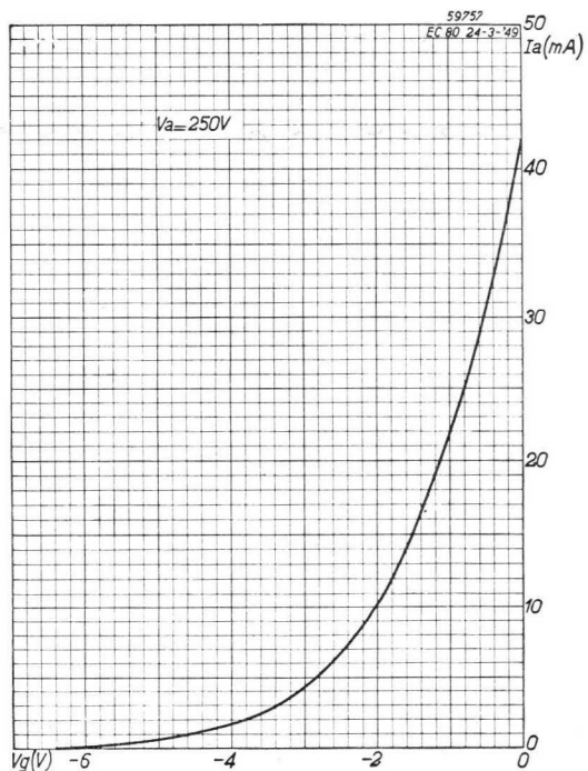
Fig.6. I_{\alpha}/V_g characteristic of the EC 80 at an anode voltage of 250 V.
