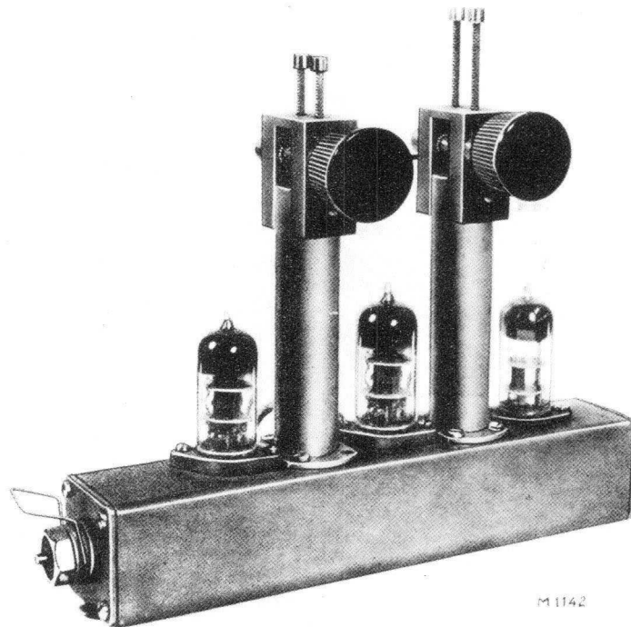
Fig.9. H.F. section of a receiver for 300 to 400 Mc/s ( \lambda = 100 to 75 cm). Mounted on the chassis are two tubes EC 80 (H.F. amplifier and mixer), one tube EC 81 (local oscillator) and two variable coaxial line circuits.
