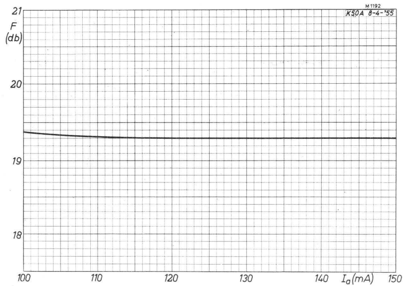
Fig.75. Noise level ( F ) of the K50A with respect to 300^\circ\text{K} as a function of the anode current.
