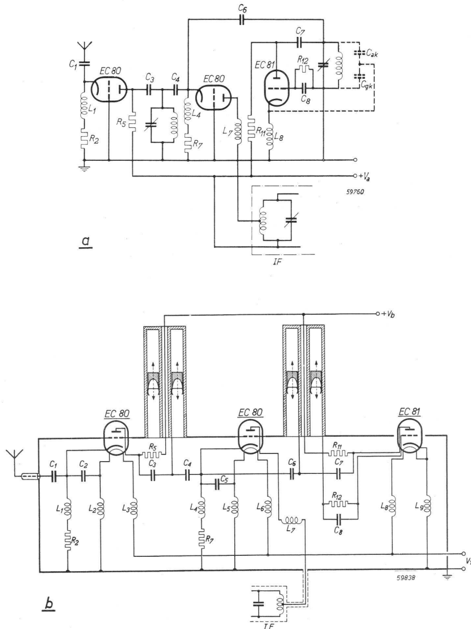
Fig.10. Circuit diagram of the H.F. section of the receiver of fig.9; (a) in simplified form, (b) complete. The first EC 80 tube functions as a U.H.F. amplifier in grounded-grid circuit, the second one as a triode mixer in grounded-grid circuit. The EC 81 tube operates as an oscillator. R_2 and R_7 of 100 \Omega each are resistors for automatic positive cathode voltage (with respect to the grid connected to earth). R_5 and R_{11} are anode resistors of 1000 \Omega each. R_{12} is the oscillator grid leak of 10\,000 \Omega . C_1, C_2, C_3, C_5, C_7 = 100 \text{ pF} , C_4 = 5.6 \text{ pF} , C_6 = 2 \text{ pF} , C_8 = 56 \text{ pF} . The oscillator (EC 81) functions as a Colpitts oscillator by means of the interelectrode capacitances C_{ak} and C_{gk} (dotted in fig.10a).
