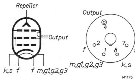
Fig.57. Electrode arrangement and base connections.
