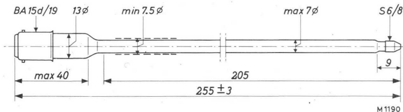
Fig.72. Dimensions in mm of the K50A.
