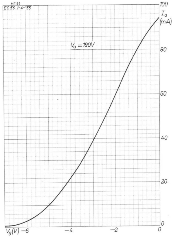
Fig. 41. I_a/V_g characteristic of the EC 56 at an anode voltage of 180 V.
