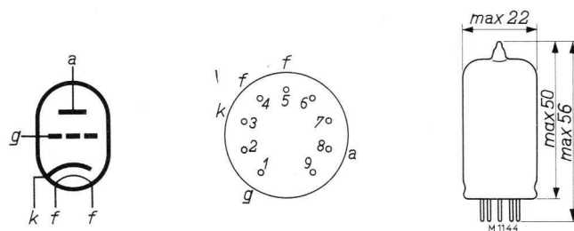
Fig. 12. Electrode arrangement, electrode connections and maximum dimensions in mm (noval base).
