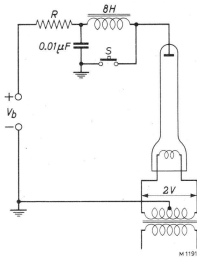
Fig.74. Recommended ignition circuit for the K50A and K51A. K50A: V_b = 500 V, R = 2700 \Omega . K51A: V_b = 350 V, R = 1000 \Omega .
