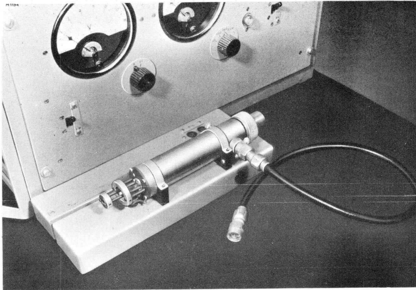
Fig.33. Photograph of an oscillator with the EC 55; frequency range from 730-1350 Mc/s.
