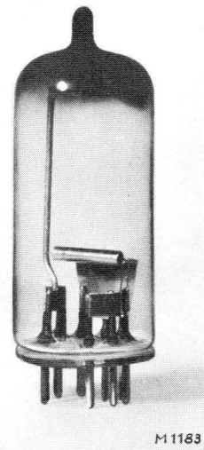
Fig.63. Photograph of the K81A (actual size).
