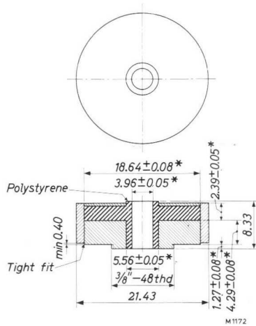
Fig. 52. Wave trap.
