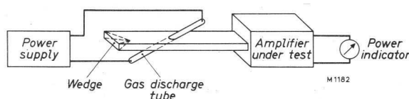
Fig.68. Outline of a microwave set-up for noise measurements.
