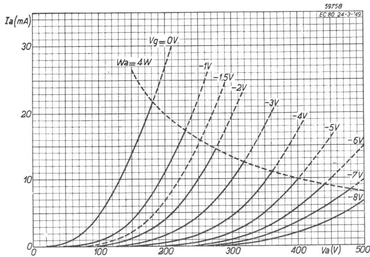
Fig.7. I_a/V_a characteristics of the EC 80. The maximum admissible anode dissipation is indicated by the dashed line W_a = 4 W.
