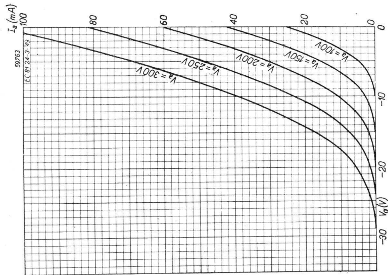
Fig. 13. I_a/V_g characteristics of the EC 81.
