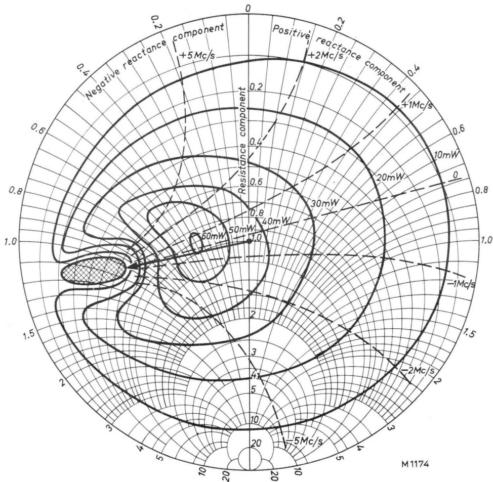
Fig.54. Typical Rieke diagram. The drawn curves are loci of constant power, and the dashed curves loci of constant frequency deviation. The sink margin is indicated by an arrow point. Within the hatched area no oscillations occur.
