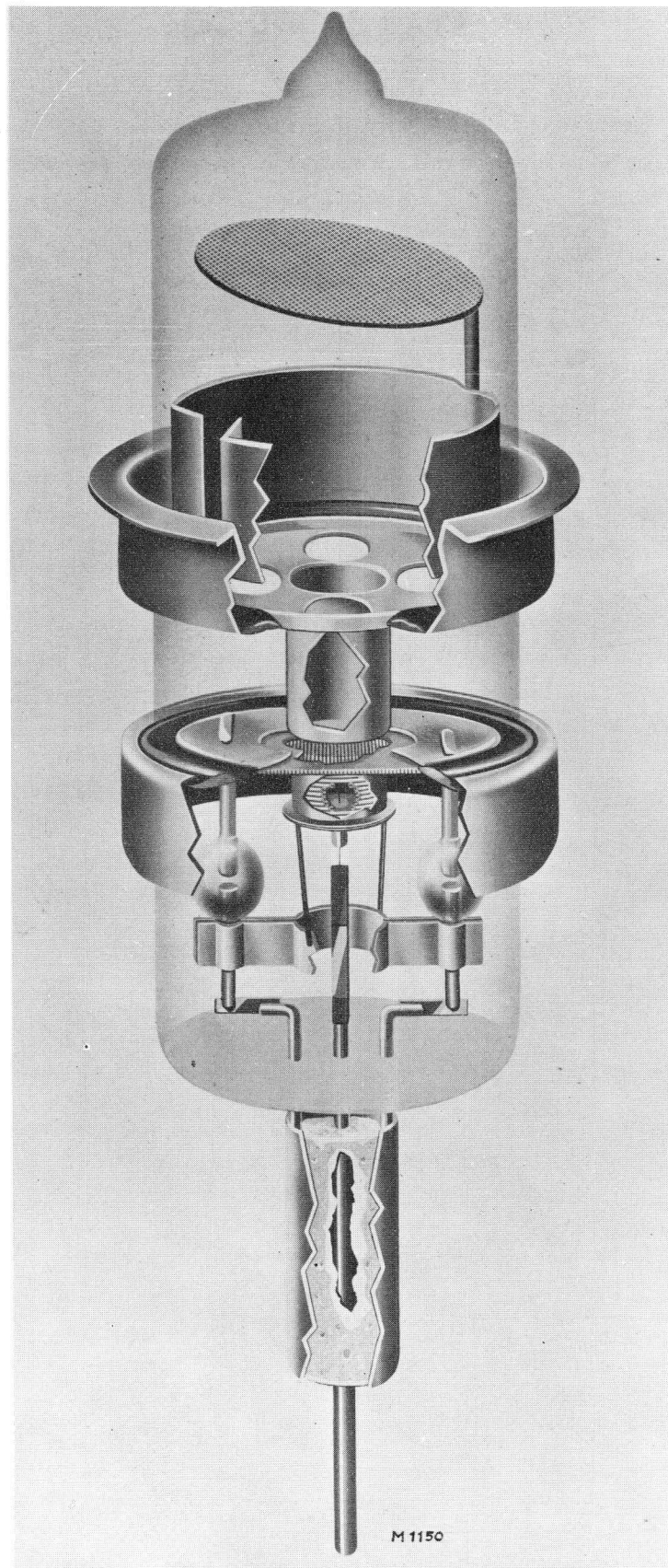
Fig. 28. Greatly enlarged representation of the EC 55.
