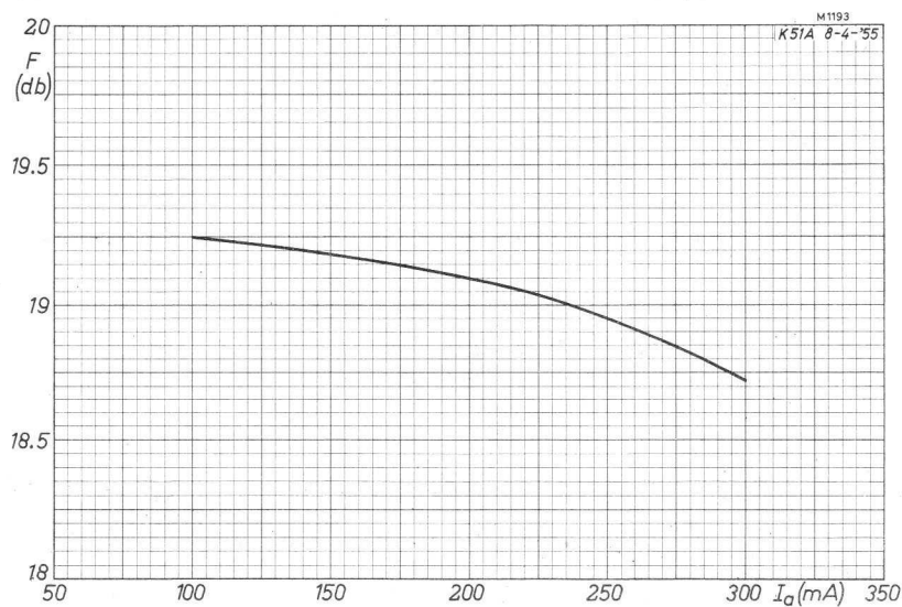
Fig.76. Noise level ( F ) of the K51A with respect to 300^\circ\text{K} as a function of the anode current.
