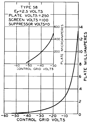
AVERAGE CHARACTERISTICS
