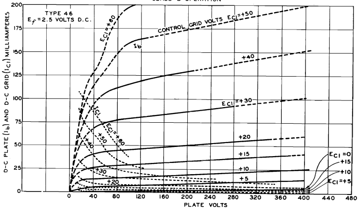
AVERAGE OPERATION CHARACTERISTICS CLASS A OPERATION
