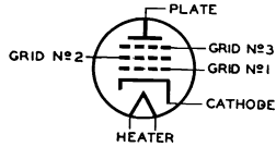
Triple-Grid Power Amplifier
