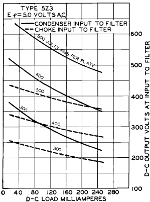
OPERATION CHARACTERISTICS
