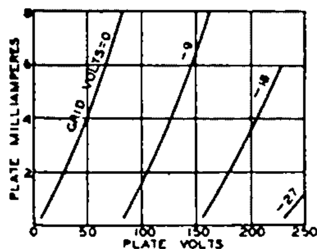
Fig. 12—Family of plate-characteristics curves.
