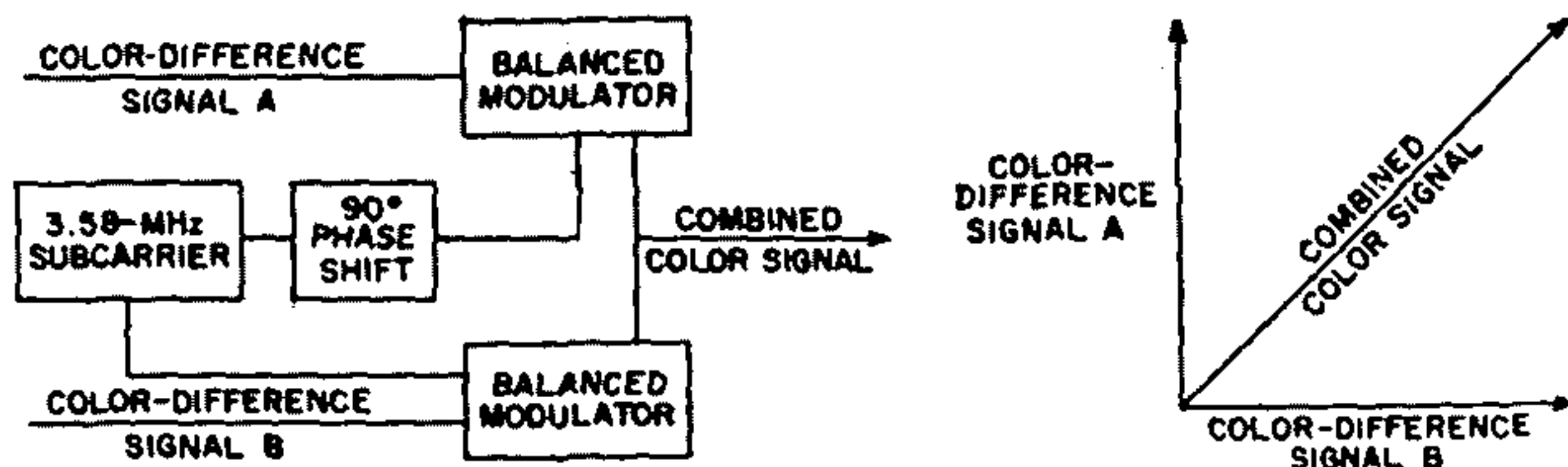
Fig. 93—Formation of combined color signal for transmission.
