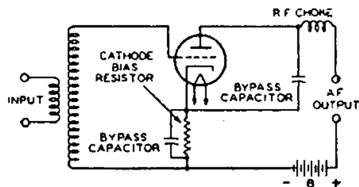
Fig. 26—Grid-bias detector circuit.
