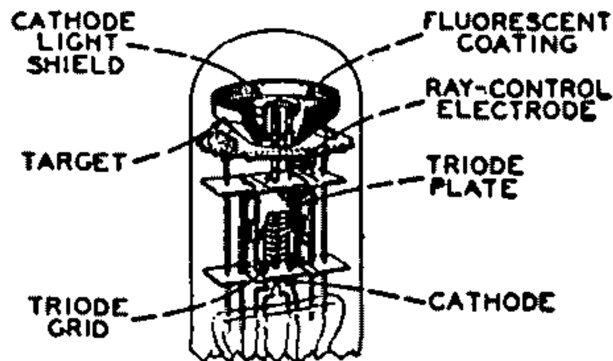
Fig. 109—Structure of electron-ray tube.
