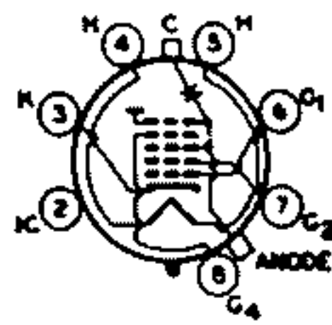
81P ANODE = G 3 + G 4 + C FOCUSING ELECTRODE - G 4
