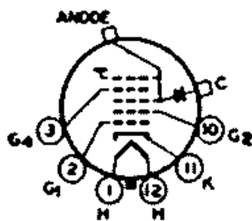
12AB ANODE = G 3 + G 4 + C FOCUSING ELECTRODE - G 4
