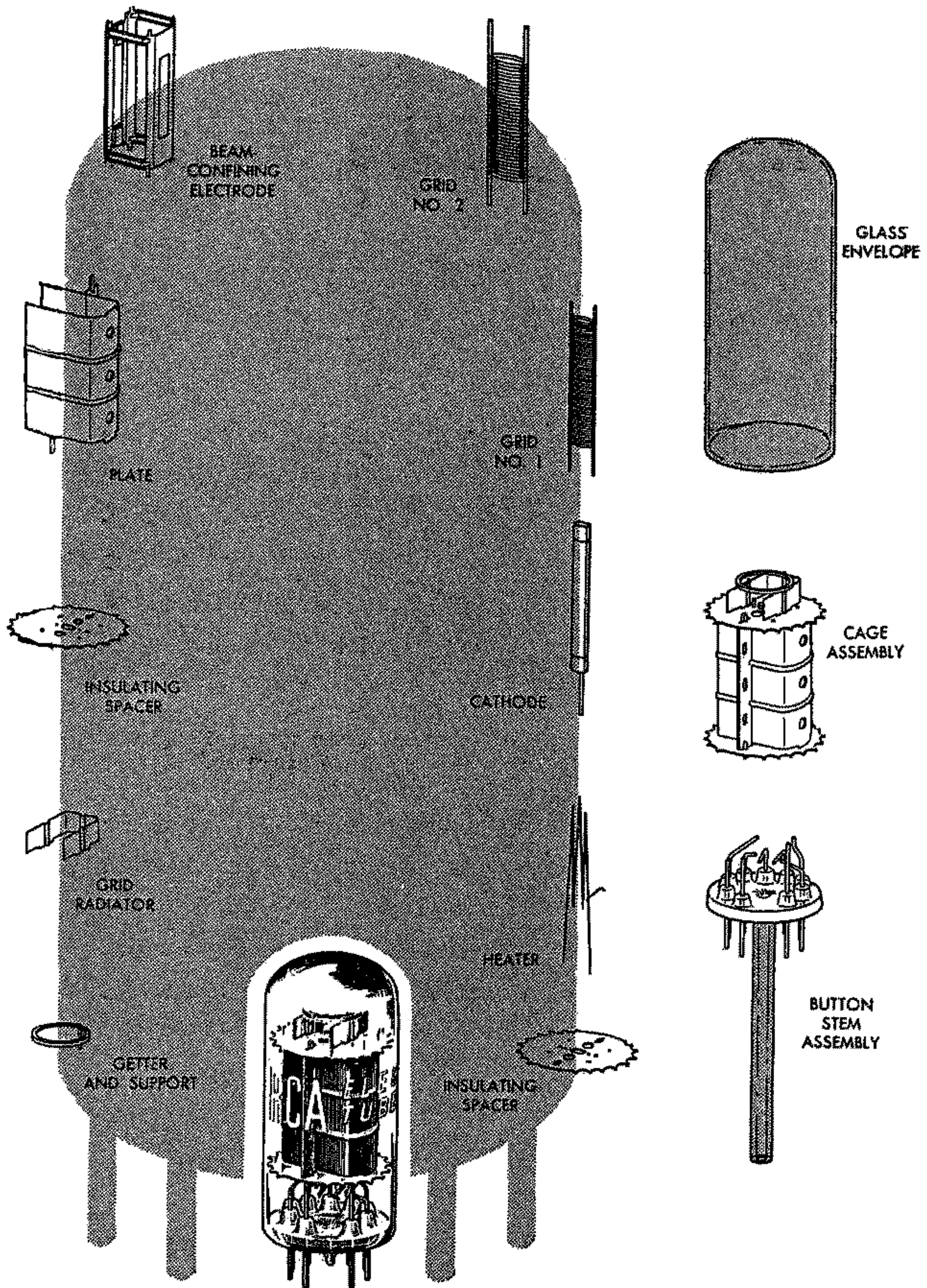
PARTS OF A NOVAR TUBE
