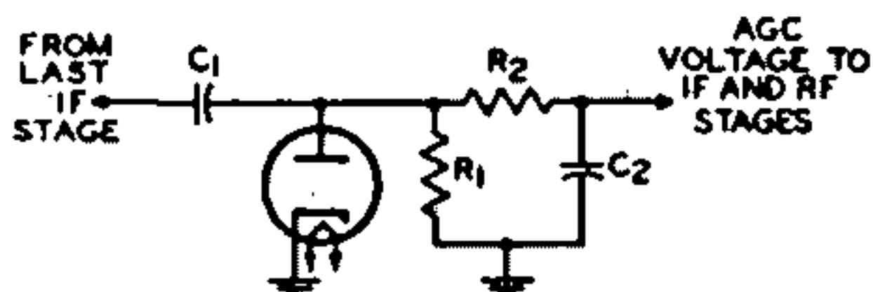
Fig. 63—Automatic-gain control (agc) circuit.
