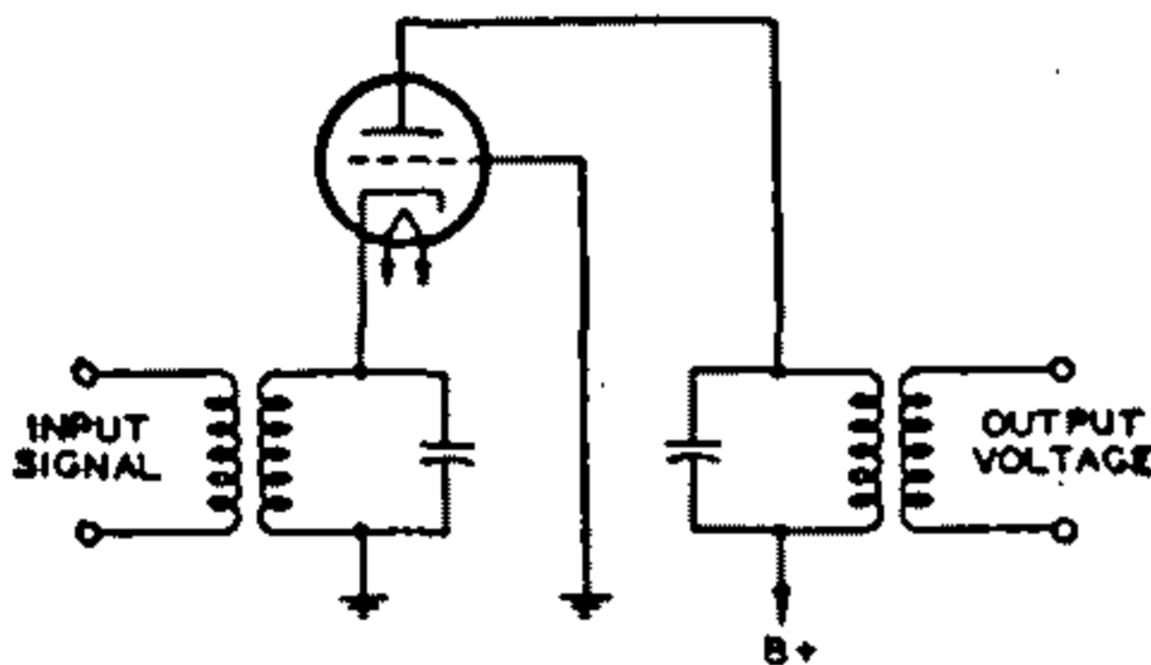
Fig. 47—Cathode-drive circuit.
