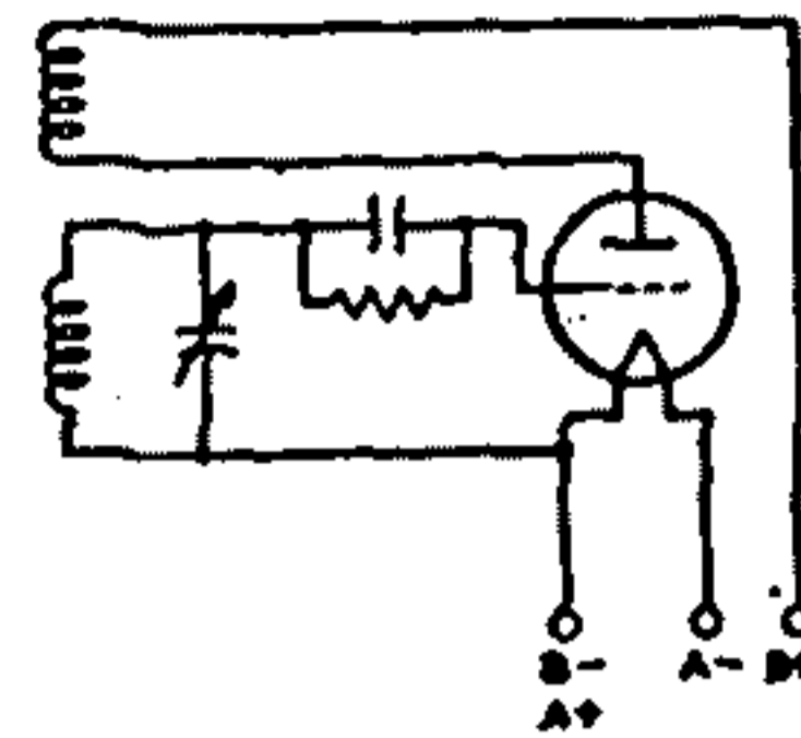
Fig. 98—Tuned-grid triode oscillator circuit using filament-type tube.
