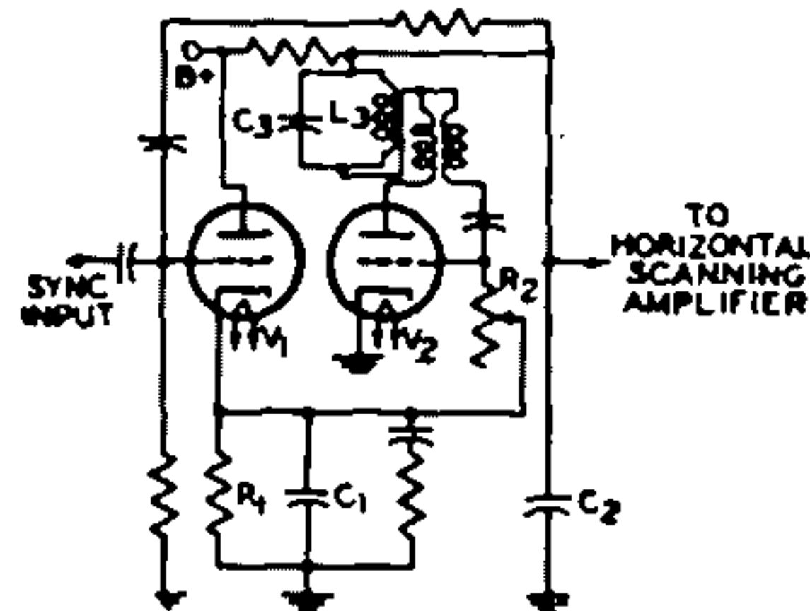
Fig. 101—Simplified synchroguide circuit.
