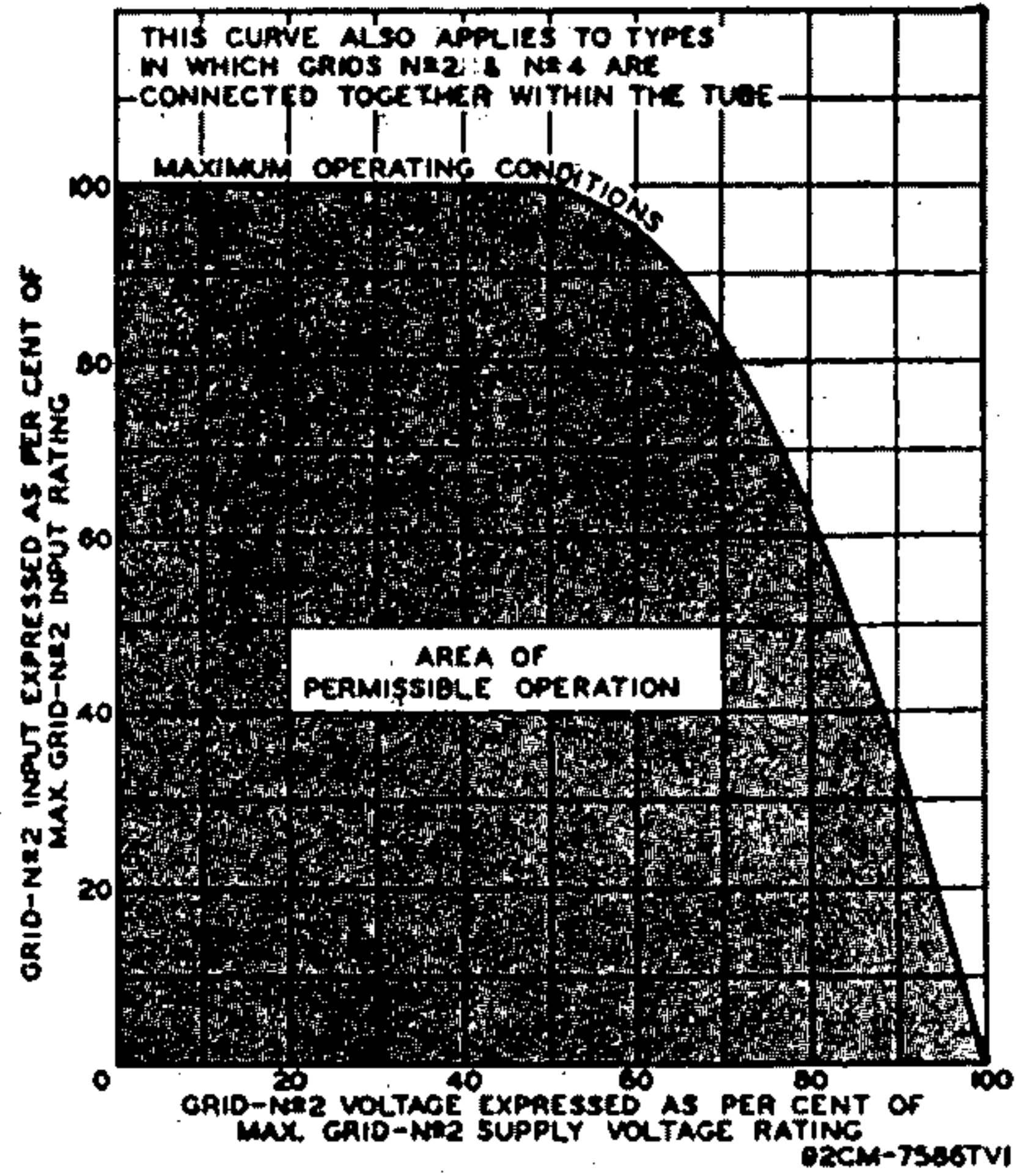
Fig. 128—Grid-No. 2 input rating curve.
