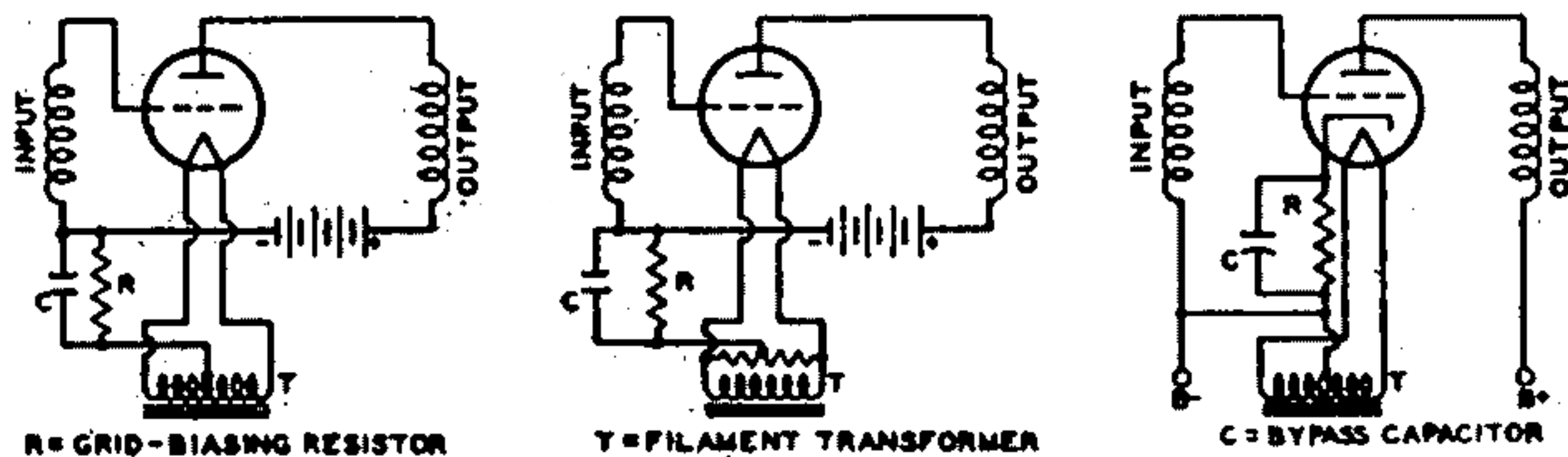
Fig. 113—Typical grid-voltage supply circuits.
