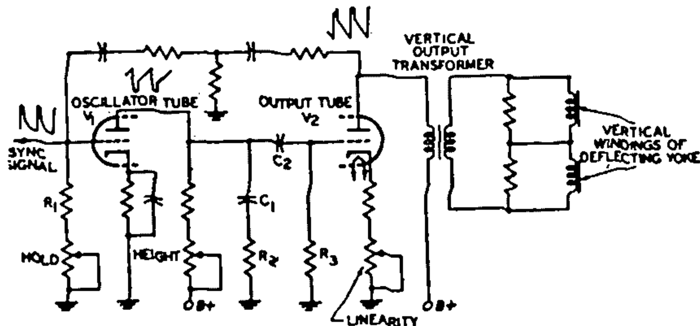
Fig. 90—Simplified combined vertical-oscillator-and-output stage.
