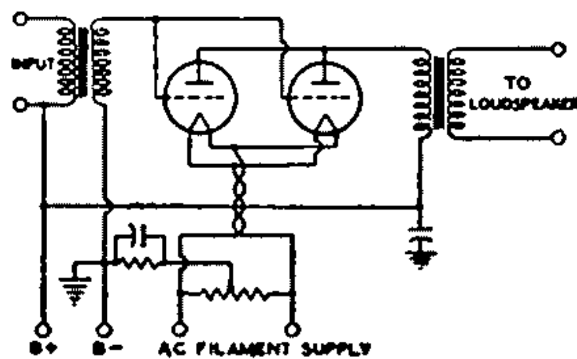
Fig. 39—Power amplifier with tubes connected in parallel.
