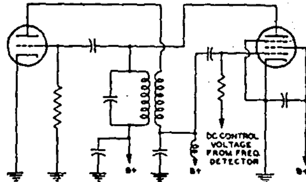
Fig. 104—Automatic-frequency-control (afc) circuit.
