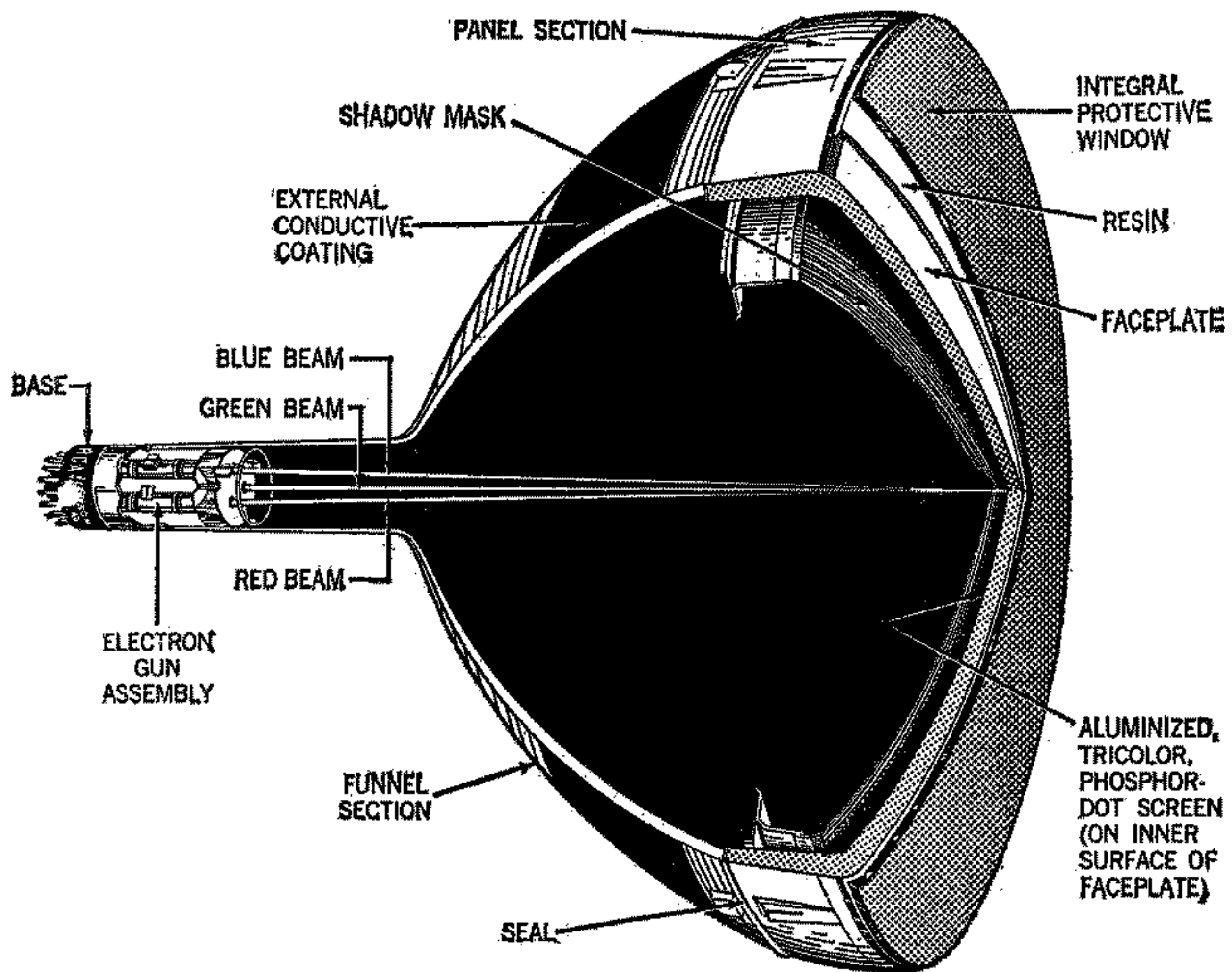
Fig. 11—Cutaway view of color television picture tube.
