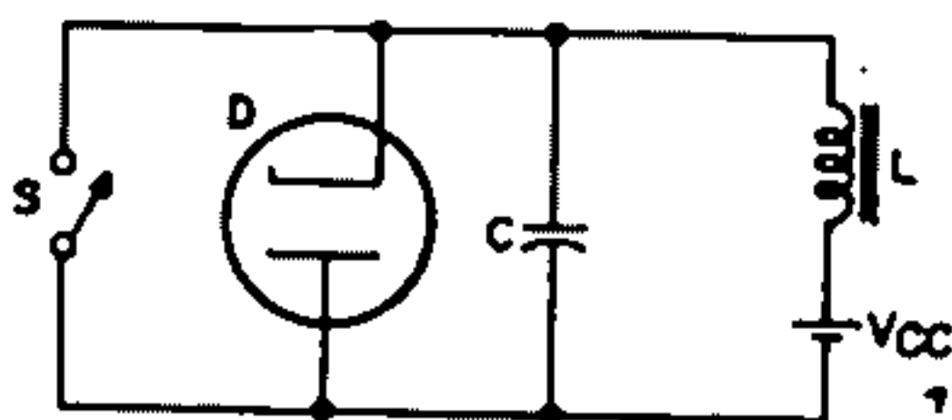
Fig. 88—Incorporation of damper diode.
