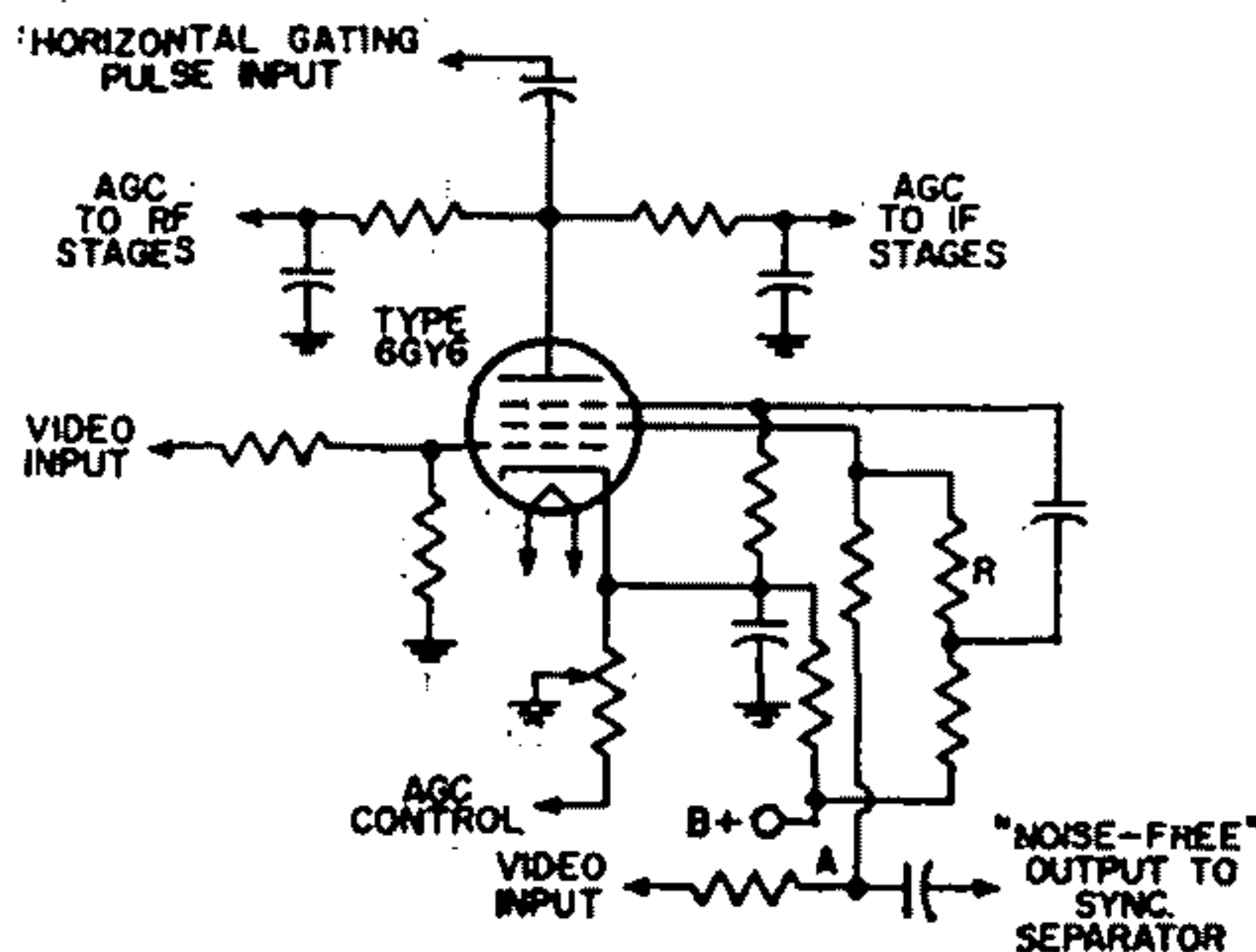
Fig. 84—Typical noise-cancellation circuit.
