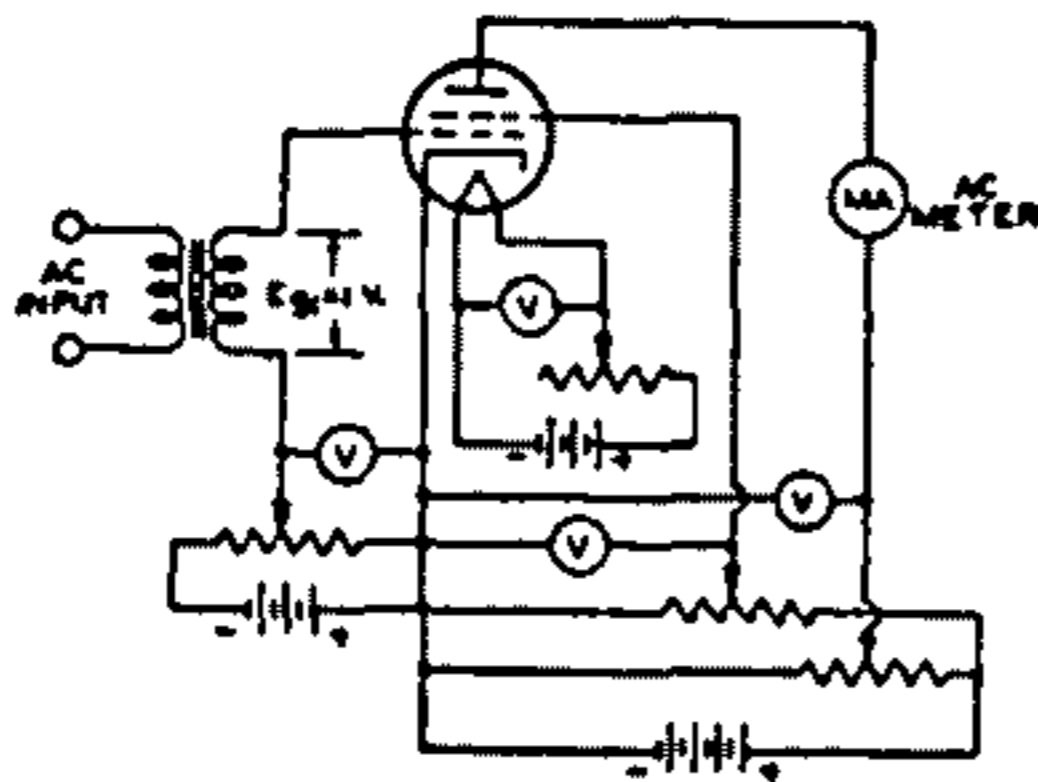
Fig. 132—Fundamental circuit of a dynamic transconductance tester.
