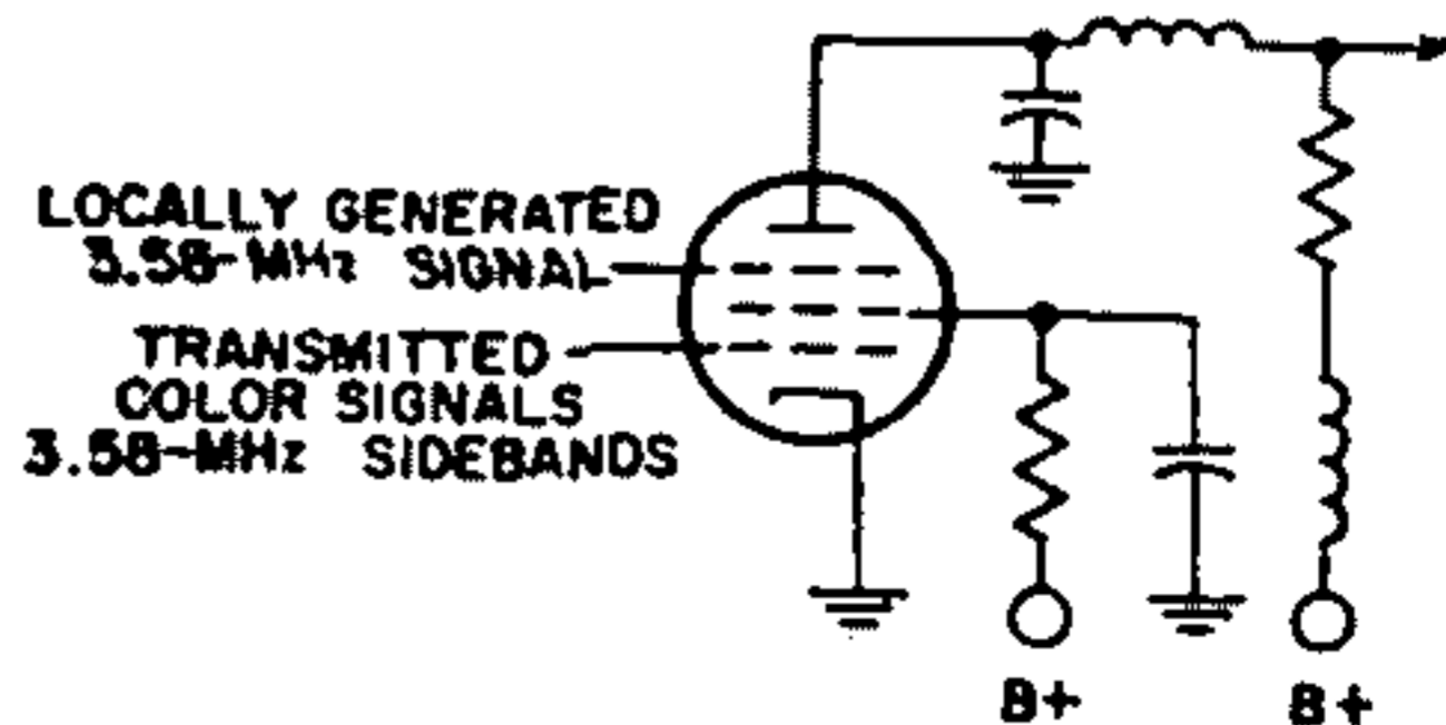
Fig. 96—Low-level color demodulator.
