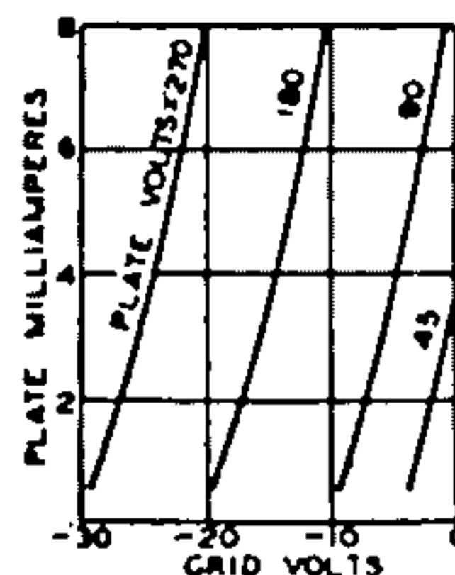
Fig. 13—Family of transfer-characteristics curves.
