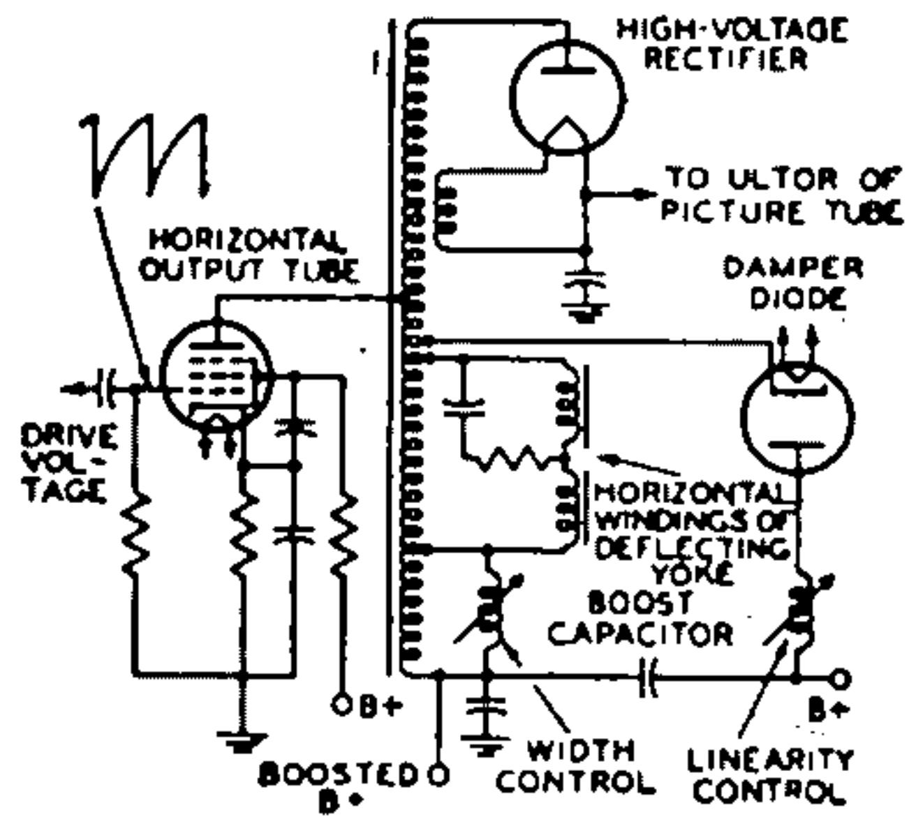
Fig. 89—Typical horizontal-deflection and high-voltage circuit.
