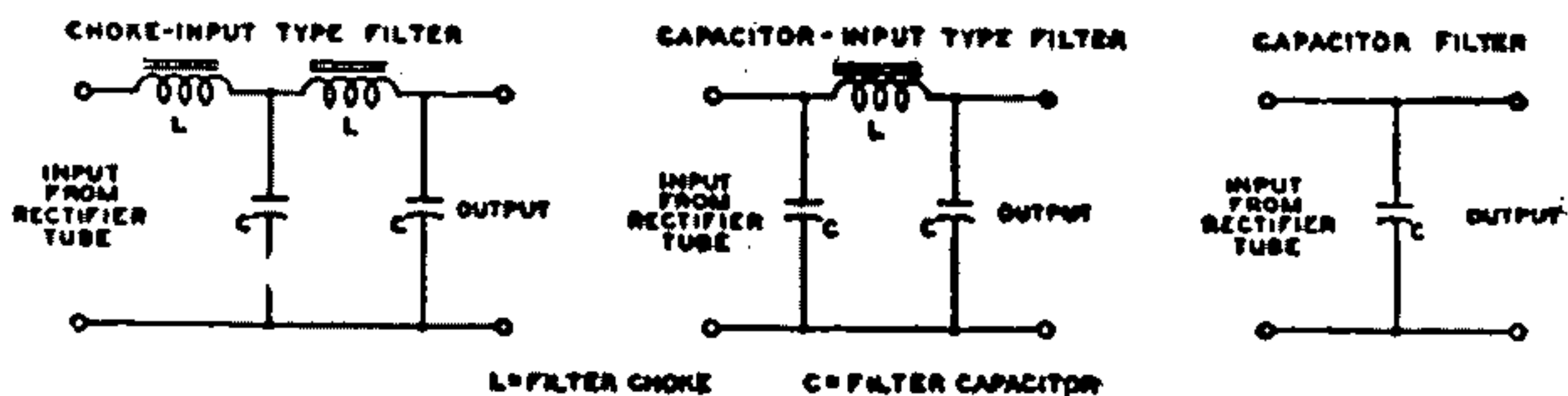
Fig. 121—Typical smoothing filters for rectifier tubes.
