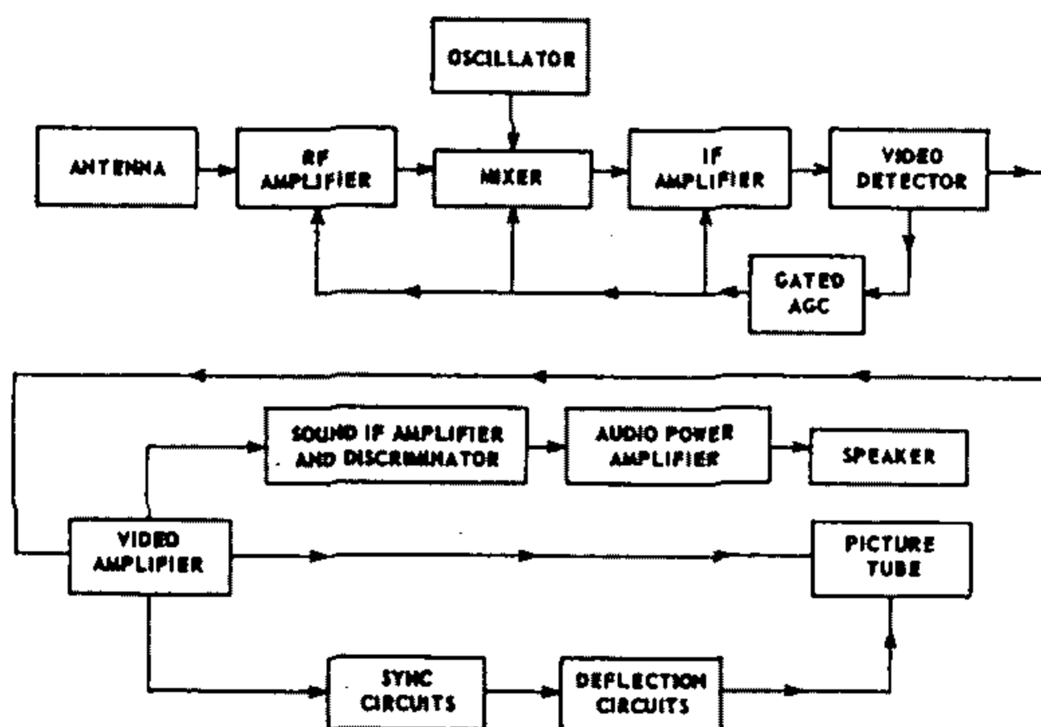
Fig. 15—Simplified block diagram for a television receiver.
