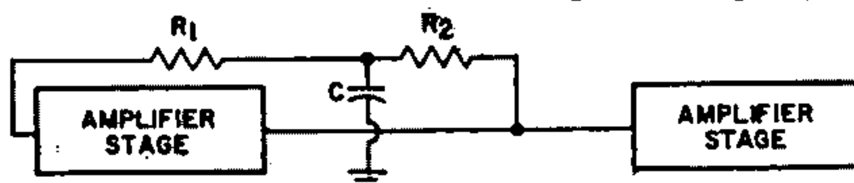
Fig. 55—Negative-feedback frequency-compensation network.
