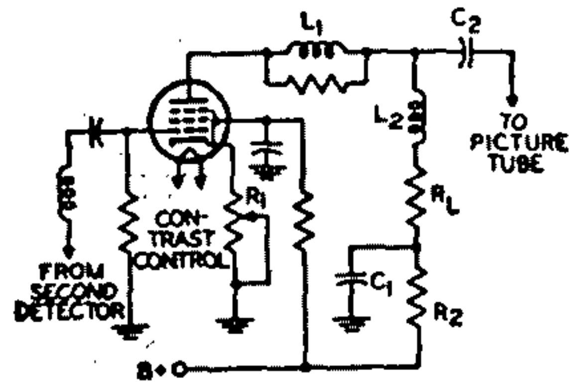
Fig. 76—Typical video amplifier stage.
