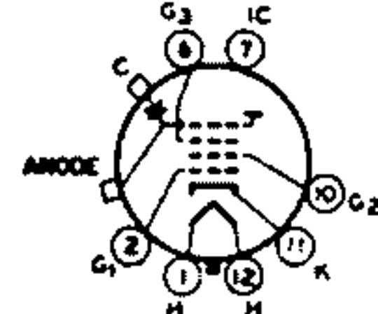
12C ANODE = G 4 + C FOCUSING ELECTRODE - G 3
