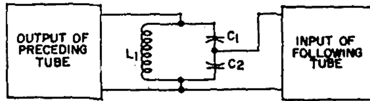
Fig. 71—Single-tuned coupling network using capacitive division.
