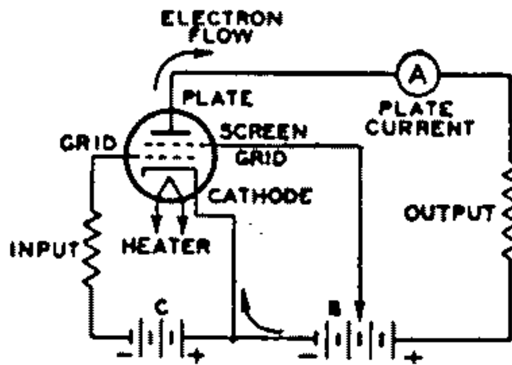
Fig. 7—Basic tetrode circuit.
