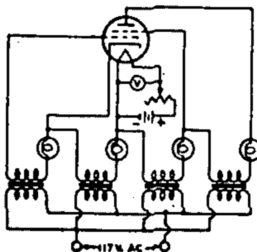
Fig. 129—Fundamental circuit of a short-circuit tester.
