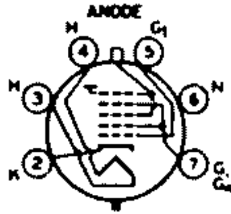
77G ANODE = G 3 + G 4 + C AUTOMATIC FOCUSING
