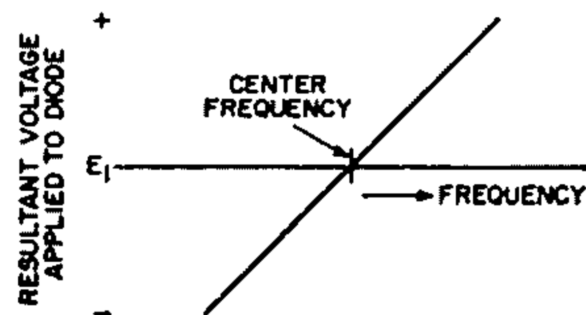
Fig. 33—Diagram showing resultant voltage E_1 in Fig. 31 as a function of frequency.
