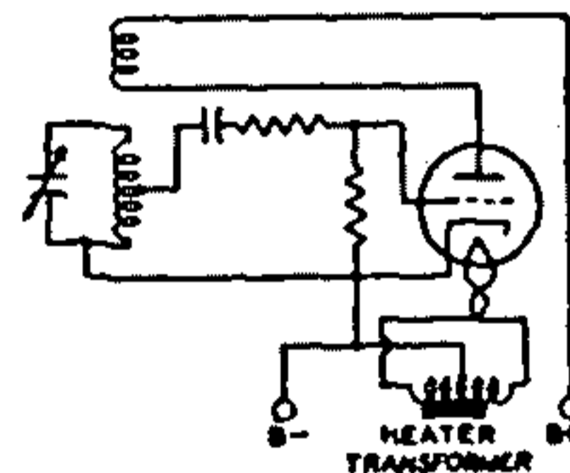
Fig. 99—Tuned-grid triode oscillator circuit using heater-cathode-type tube.
