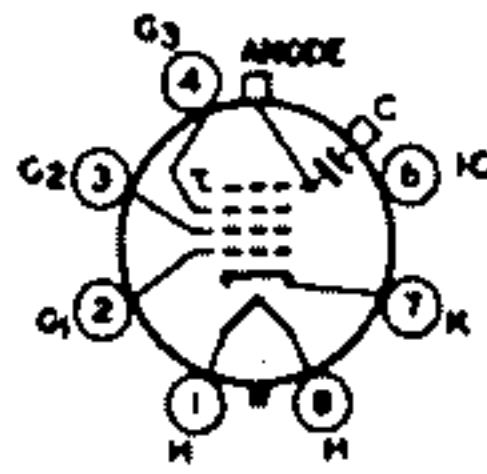
81R ANODE = G 4 + C FOCUSING ELECTRODE - G 3
