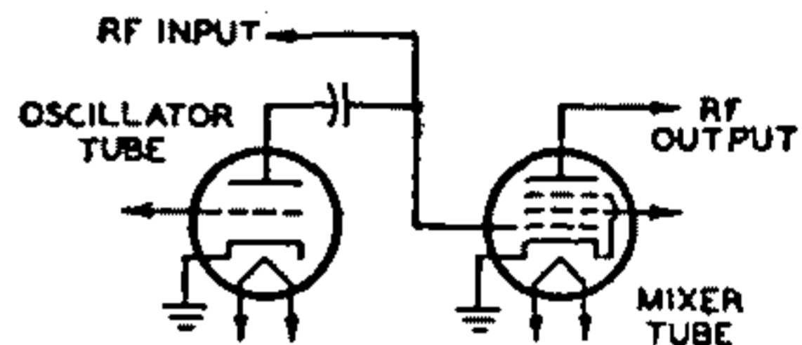
Fig. 108—Typical television mixer-oscillator circuit.
