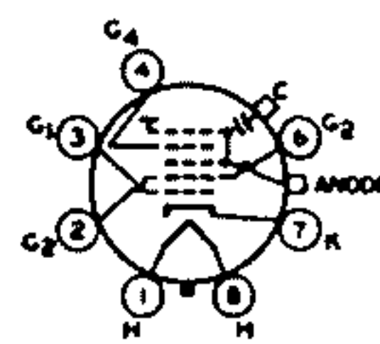
81K ANODE = G 3 + G 4 + C FOCUSING ELECTRODE - G 4
