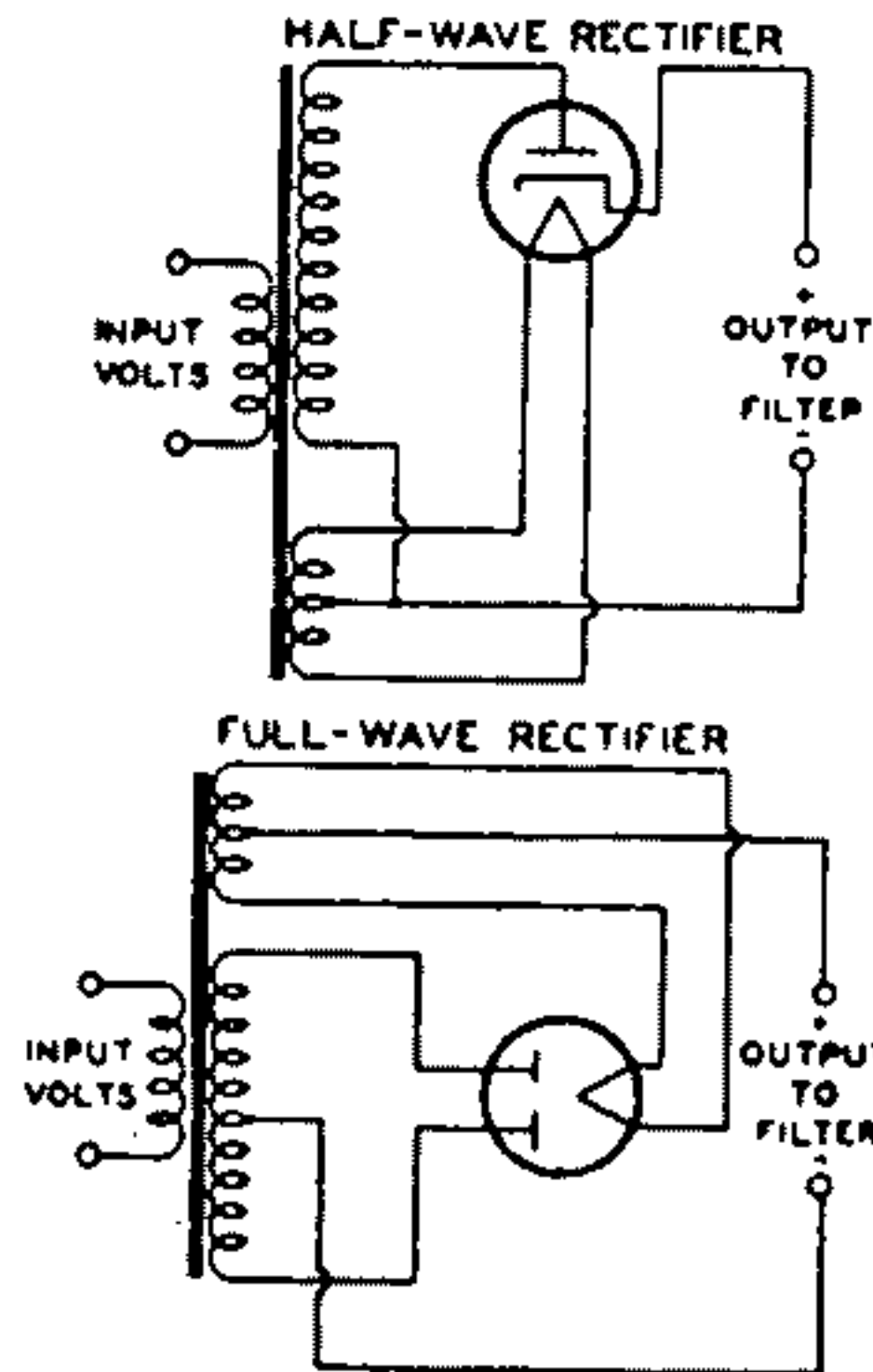
Fig. 18—Half-wave and full-wave rectifier circuits.
