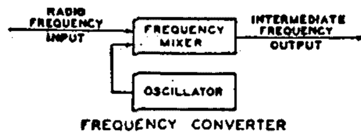
Fig. 106—Block diagram of simple frequency-converter circuit.
