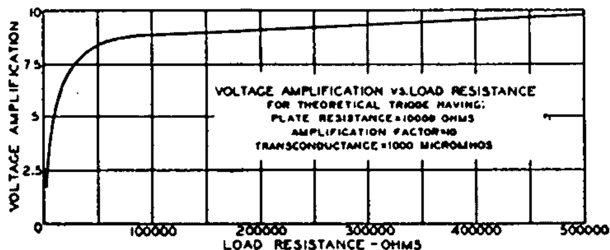
Fig. 36—Gain curve for triode amplifier circuit.
