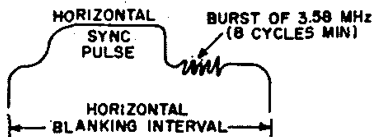
Fig. 95—Waveform for synchronizing signal.
