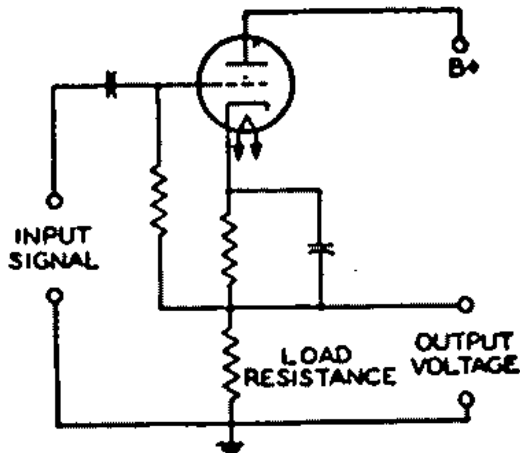
Fig. 53—Cathode-follower circuit modified for reduced bias.
