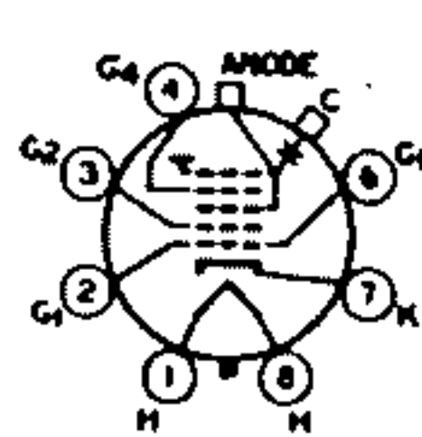
81E ANODE = G 3 + G 4 + C FOCUSING ELECTRODE - G 4
