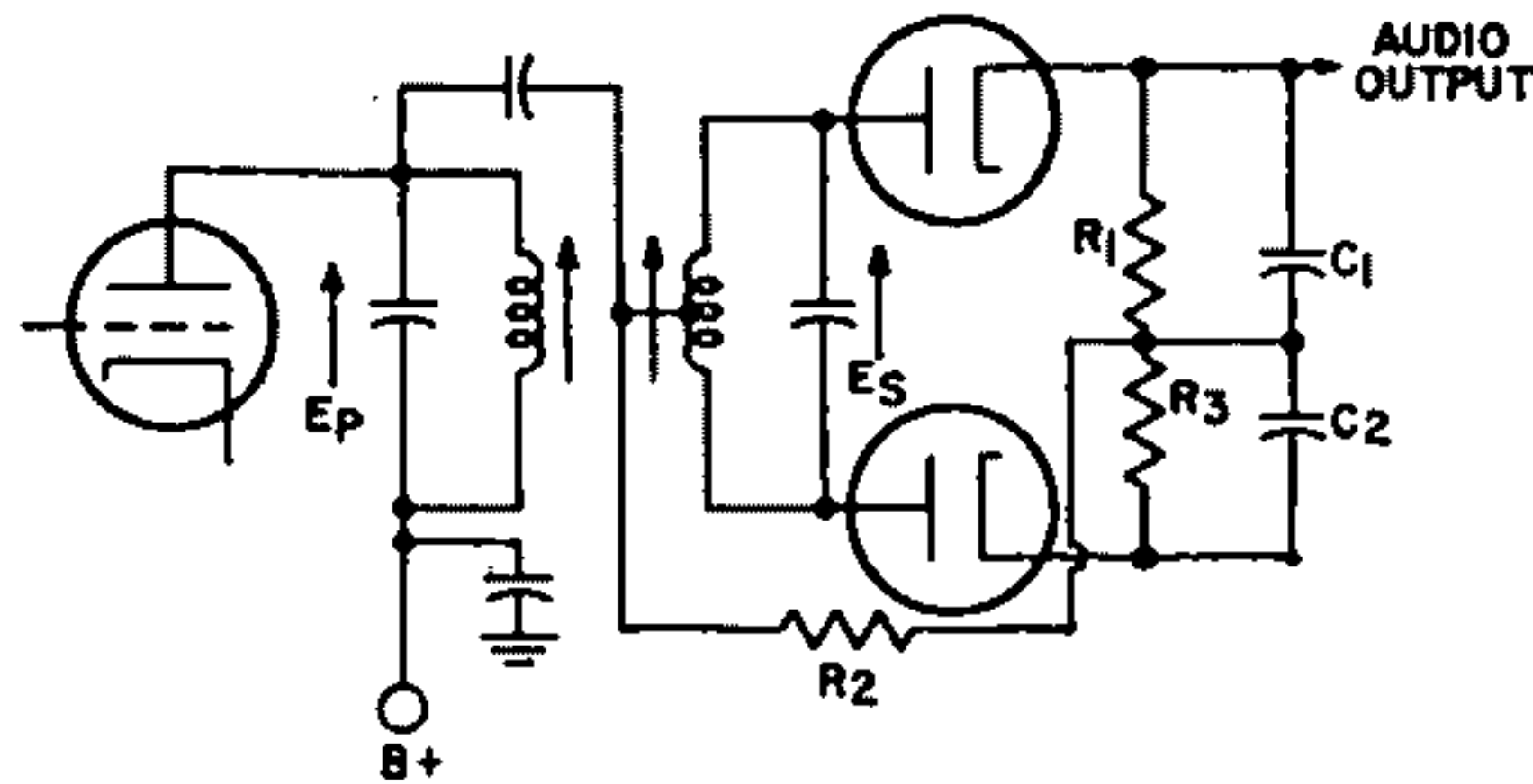
Fig. 30—Balanced phase-shift discriminator circuit.
