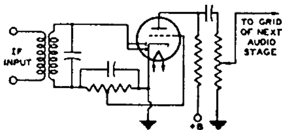
Fig. 25—Diode-biased detector circuit.
