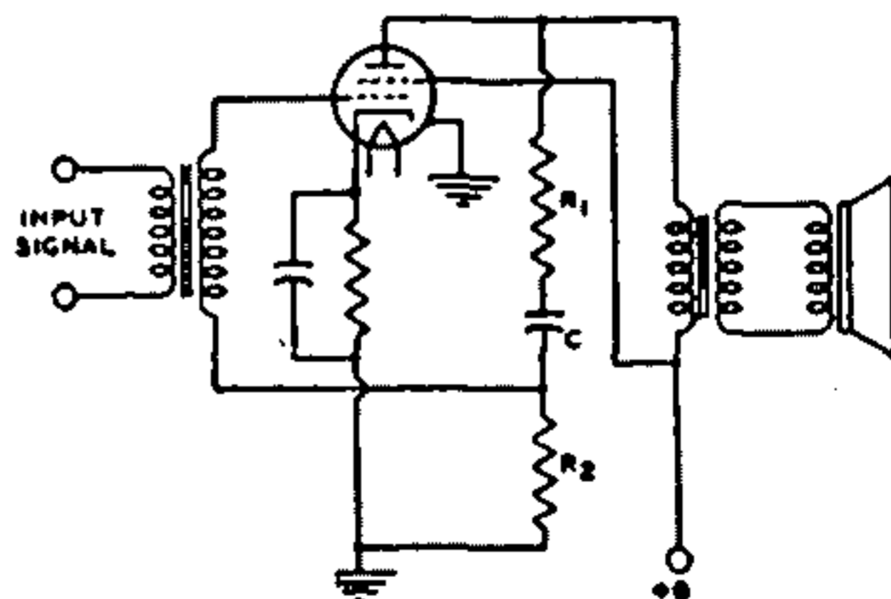
Fig. 48—Power-output stage using constant-voltage inverse feedback.
