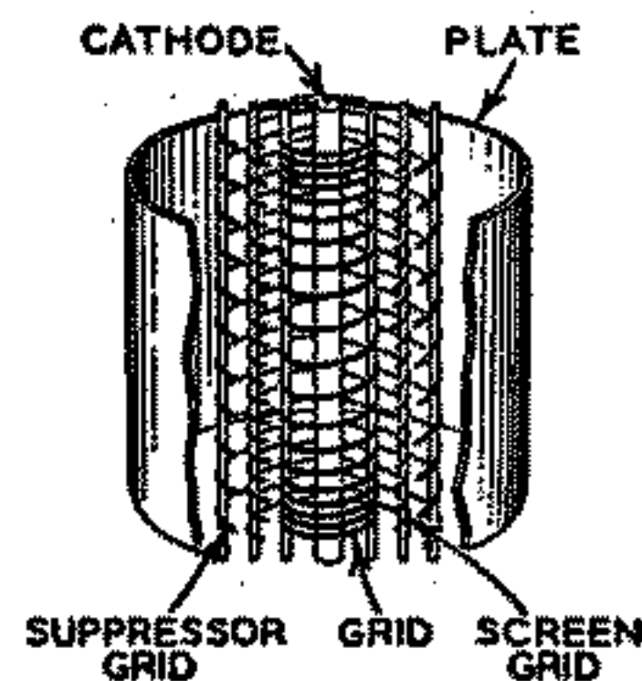
Fig. 37—Structure of remote-cutoff grid.
