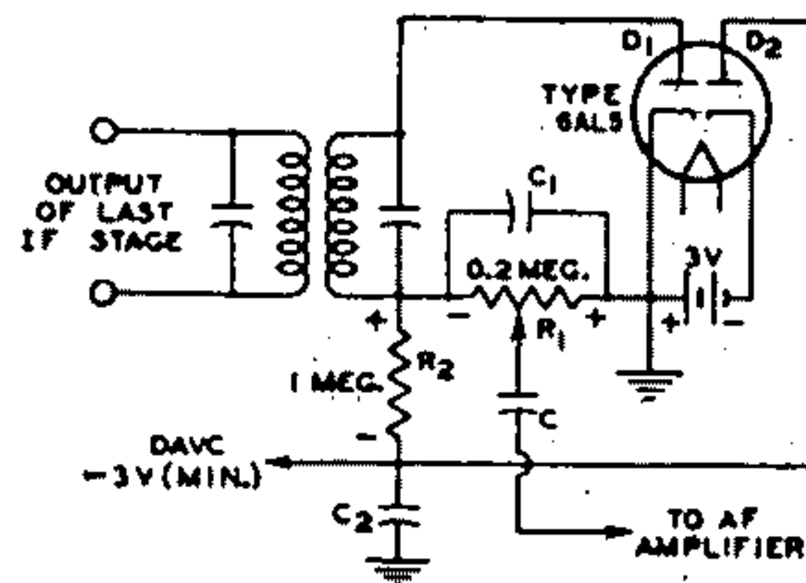
Fig. 62—Delayed avc (davc) circuit.
