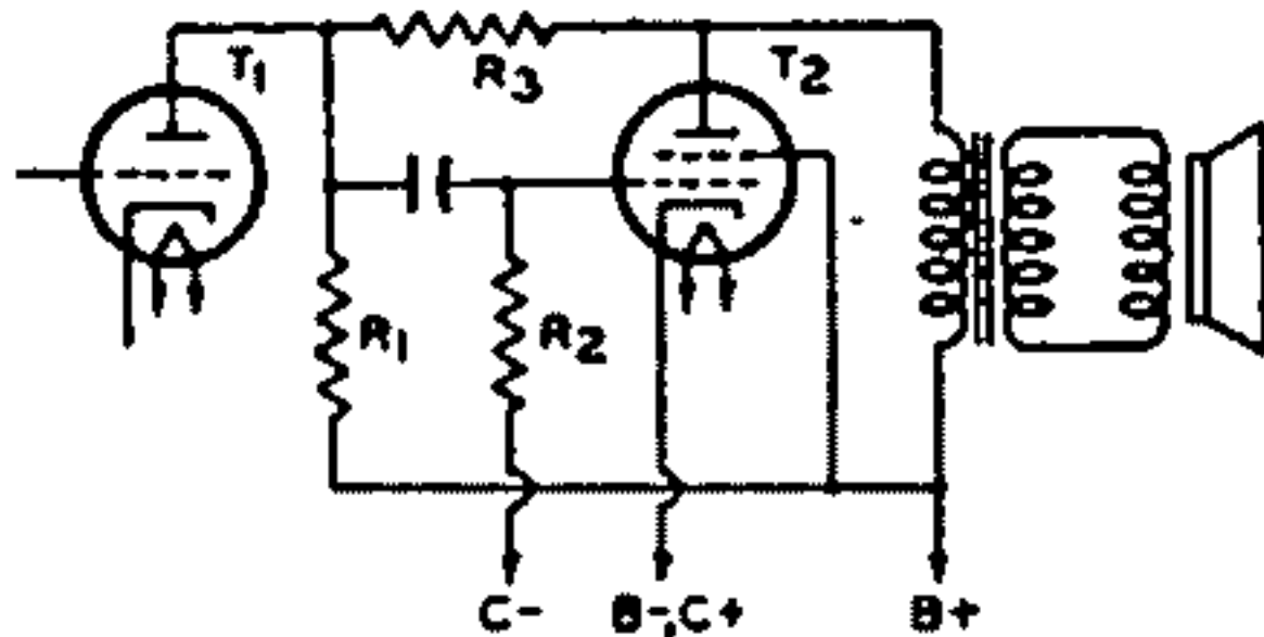
Fig. 50—Resistance-coupled stages using feedback resistor.
