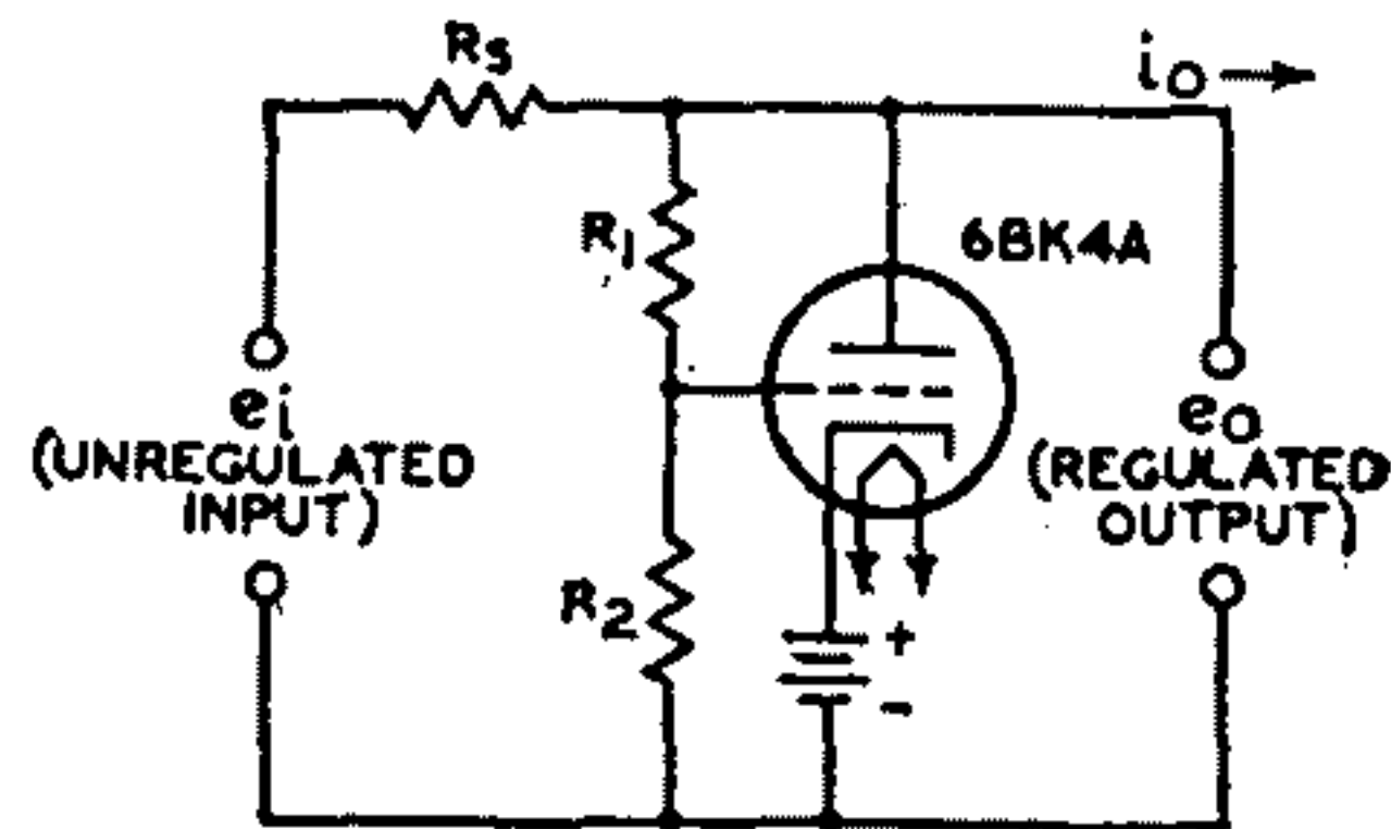
Fig. 92—High-voltage regulator circuit for color television.
