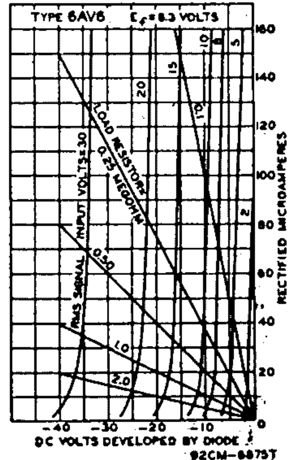
AVERAGE DIODE CHARACTERISTICS HALF-WAVE RECTIFICATION-SINGLE DIODE UNIT
