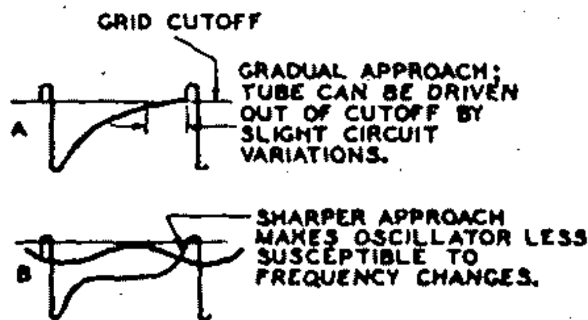
Fig. 103—Waveforms showing effect of tuned circuit L_2C_2 in Fig. 101.
