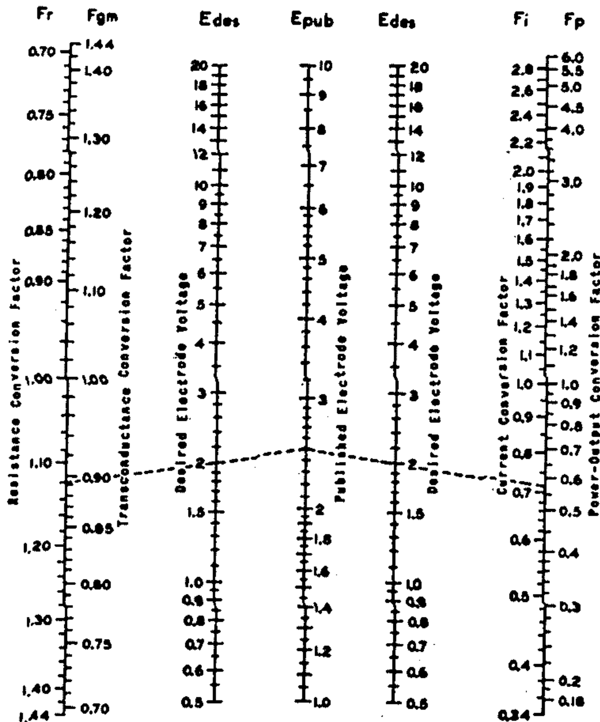
Fig. 44—Nomograph of tube conversion factors.
