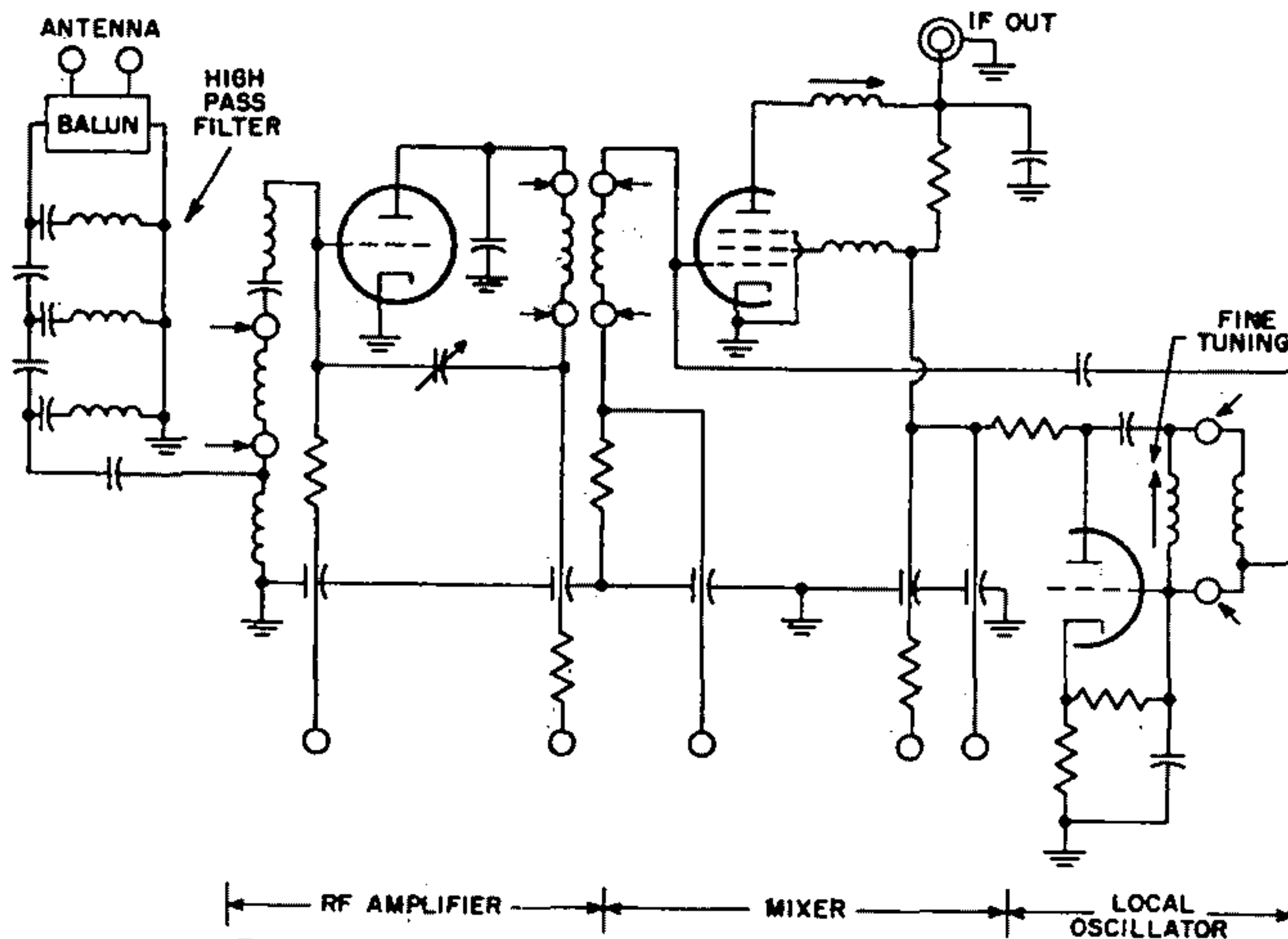
Fig. 72—Simplified schematic of typical vhf television tuner.
