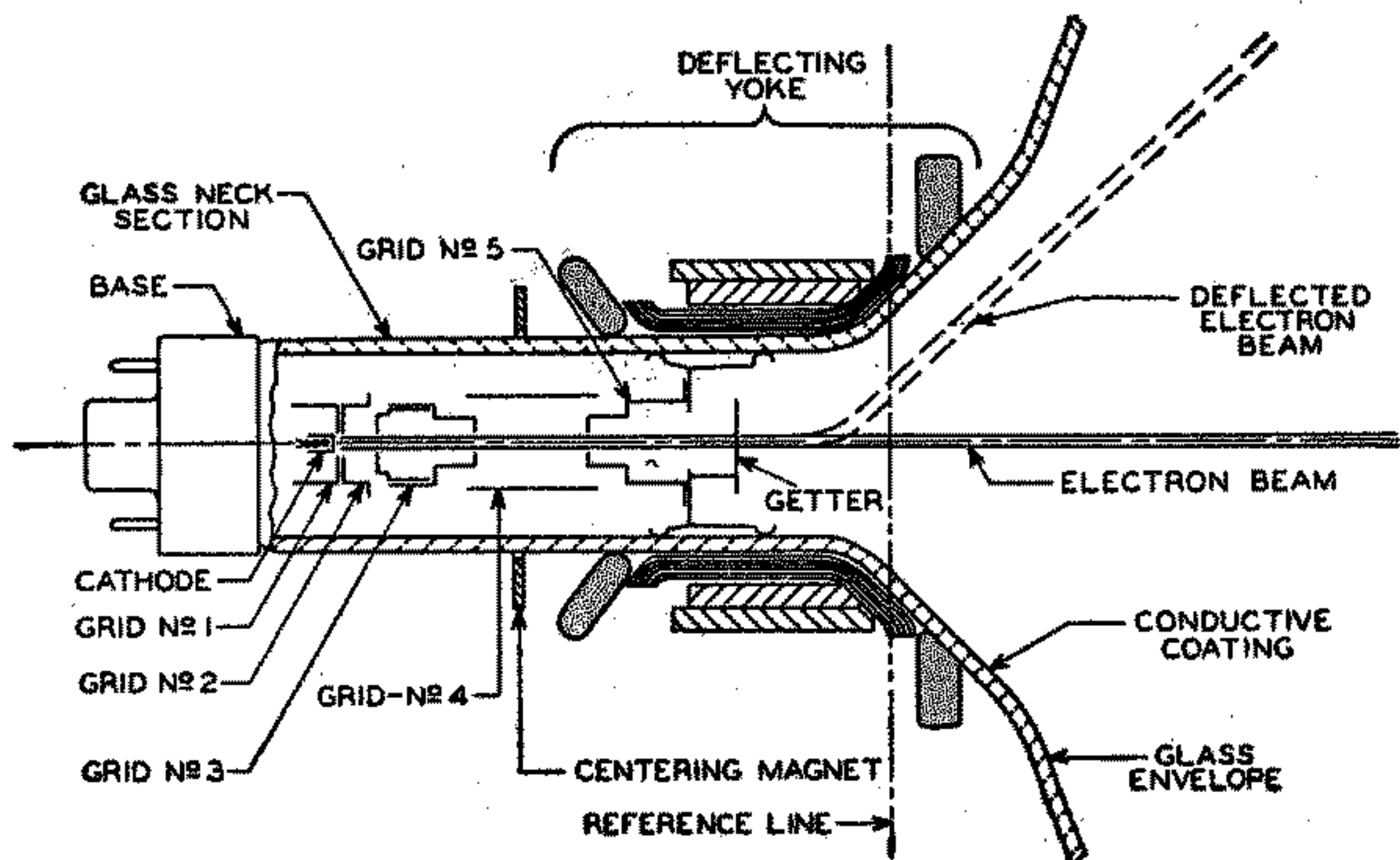
Fig. 10—Structure of television-picture-tube electron gun.
