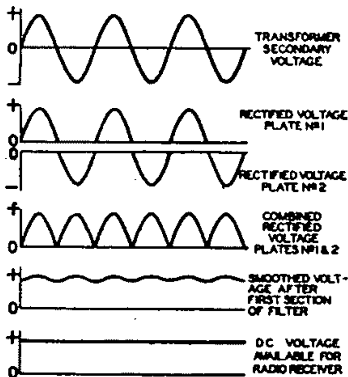
Fig. 17—Voltage waveforms of full-wave rectifier circuit.
