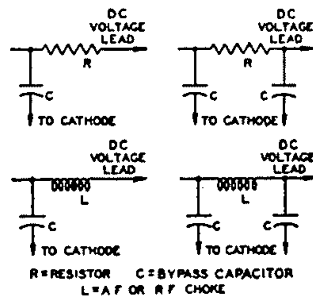
Fig. 120—Typical filter circuits.
