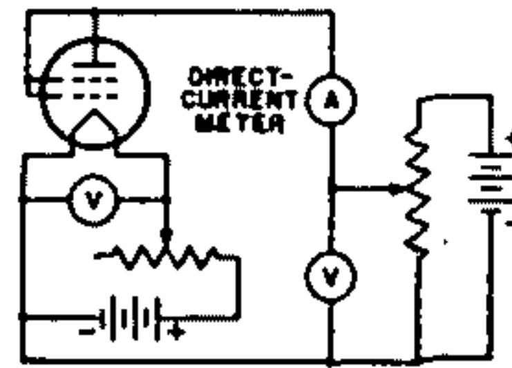
Fig. 130—Fundamental circuit of an emission tester
