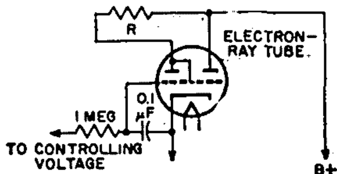
Fig. 110—Indicating circuit using an electron-ray tube.
