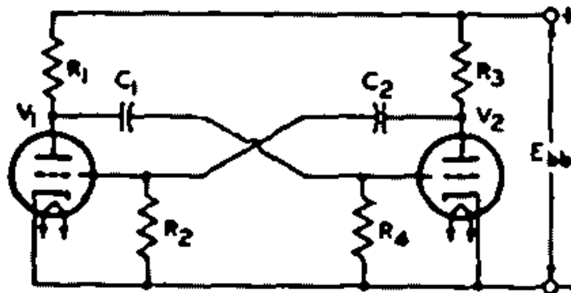
Fig. 100—Basic multivibrator circuit of the free-running type.
