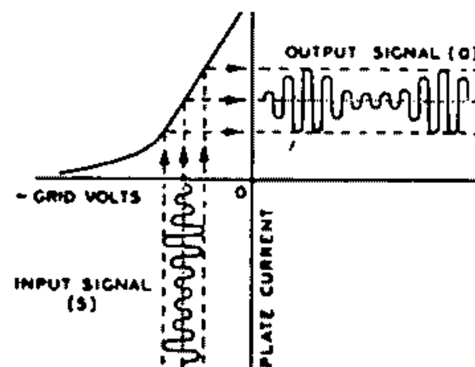
Fig. 34—Current characteristics of class A amplifier.
