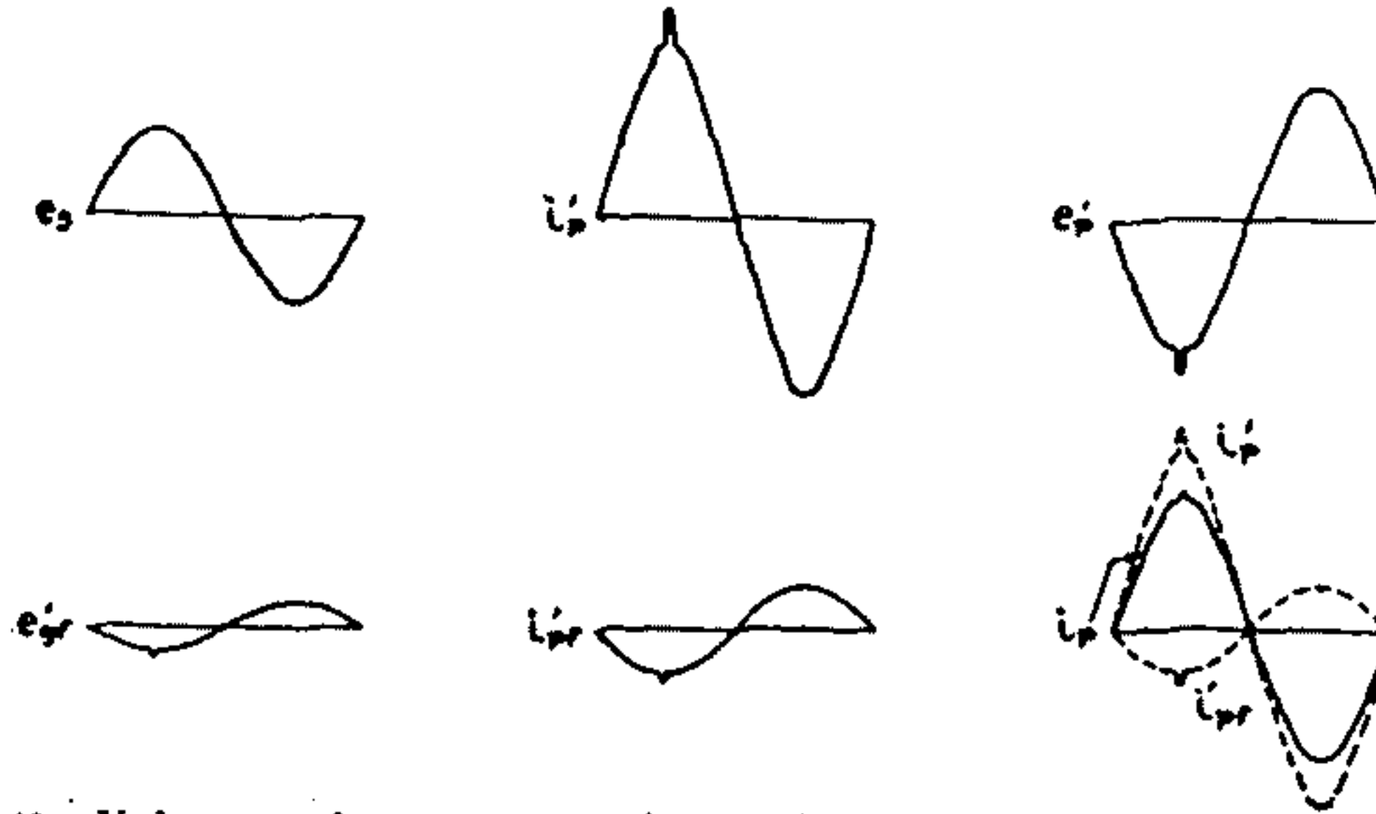
Fig. 49—Voltage and current waveforms showing effect of inverse feedback.
