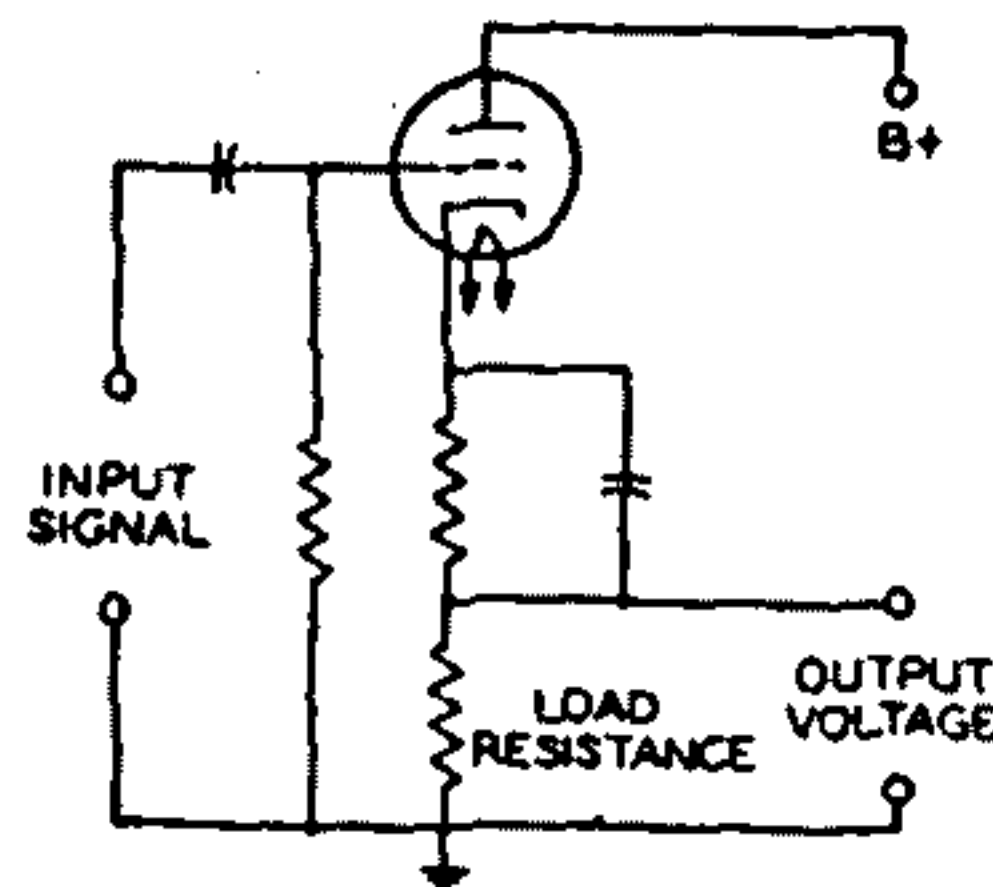
Fig. 52—Cathode-follower circuit modified for increased bias.
