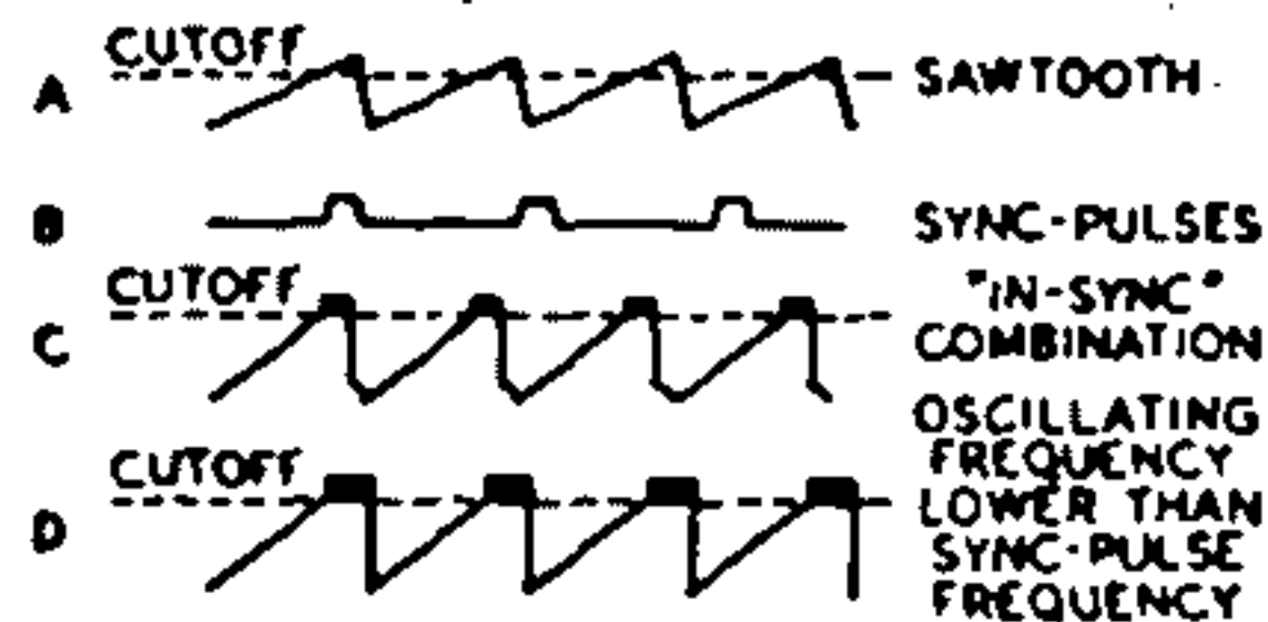
Fig. 102—Sawtooth and sync pulses in synchroguide circuit.
