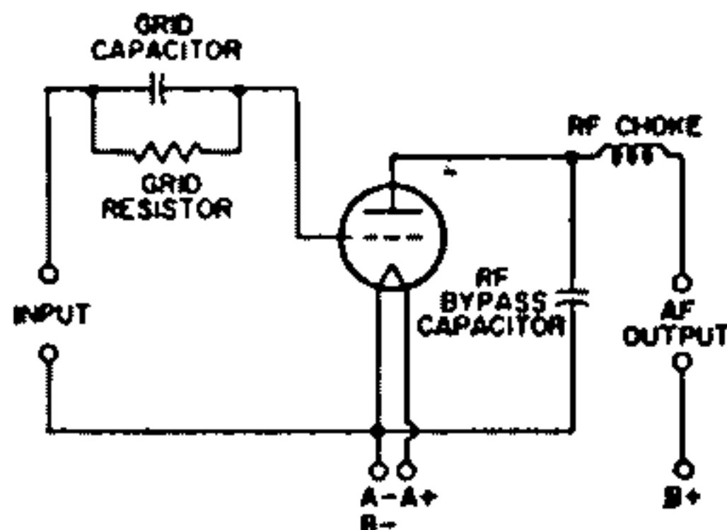
Fig. 27—Detector circuit using grid-resistor-and-capacitor bias.
