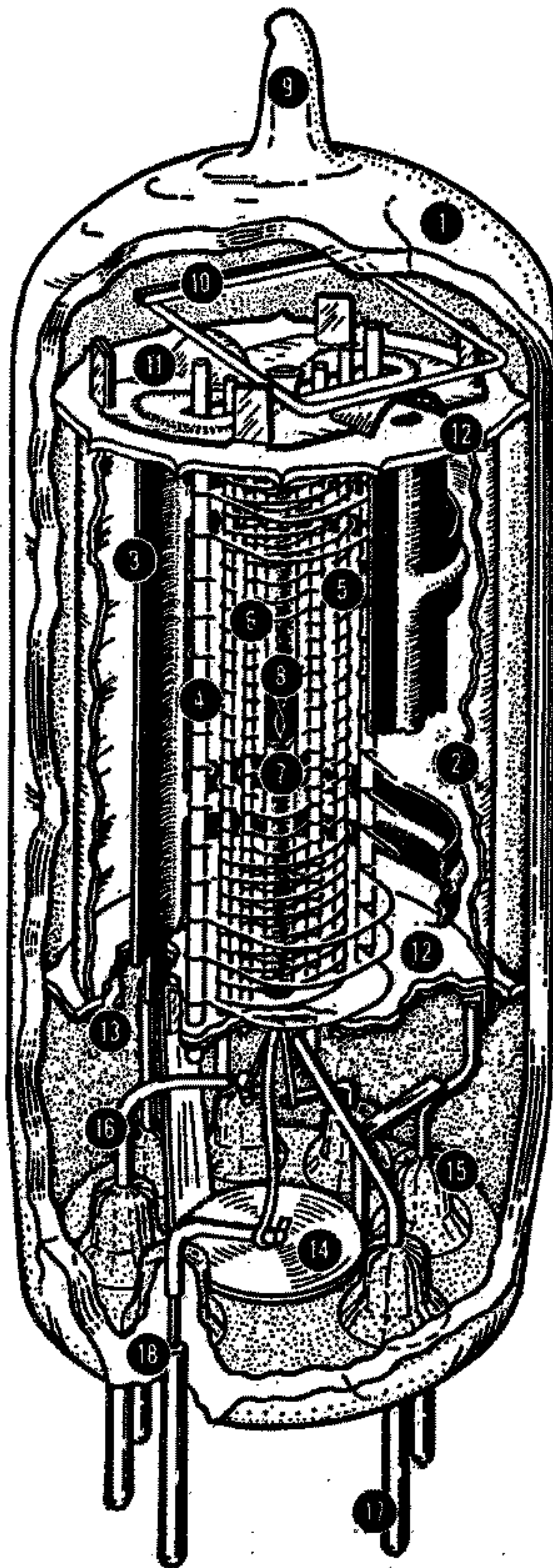
Structure of a Miniature Tube
