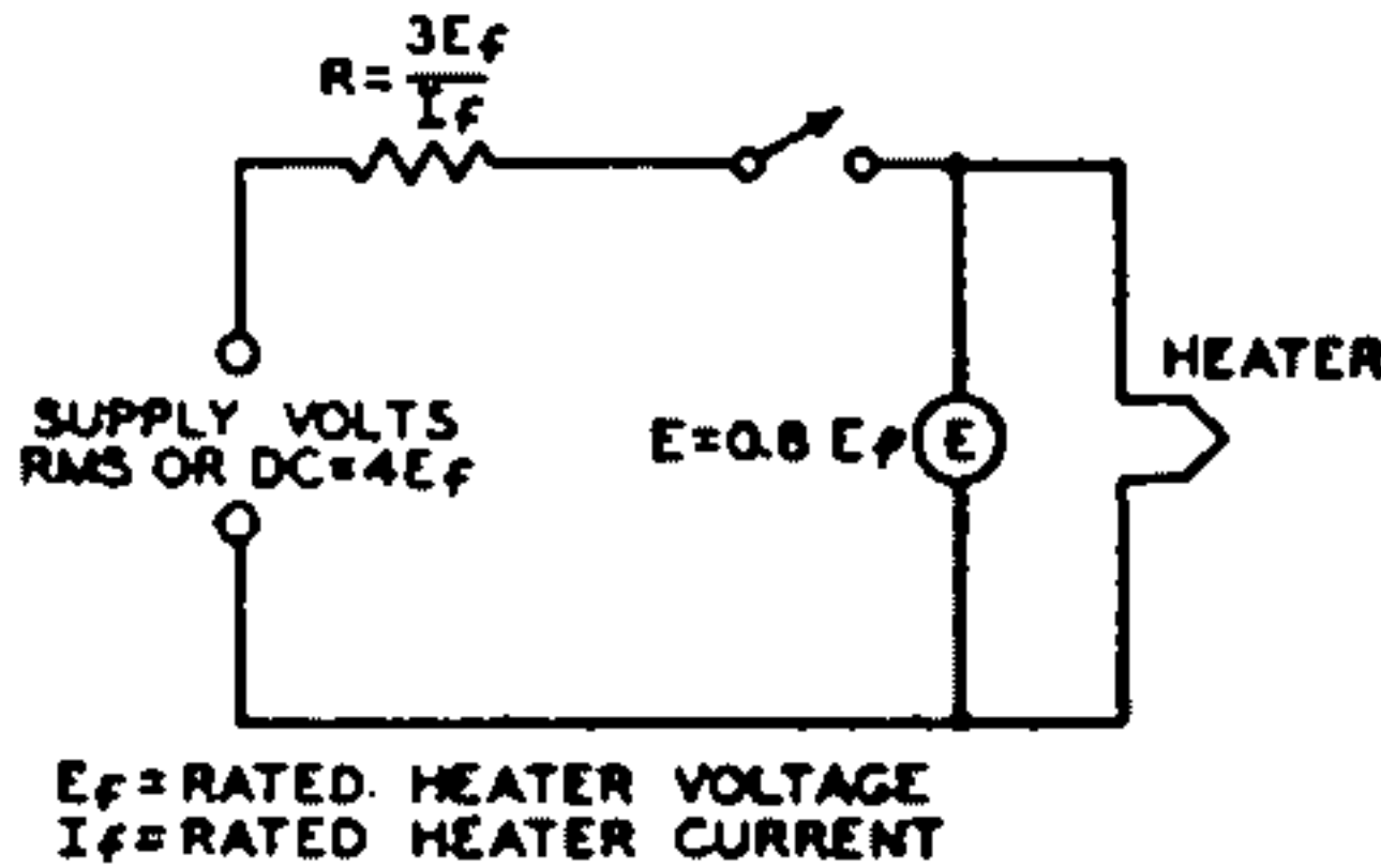
Fig. 124—Test circuit for measuring heater warm-up time.
