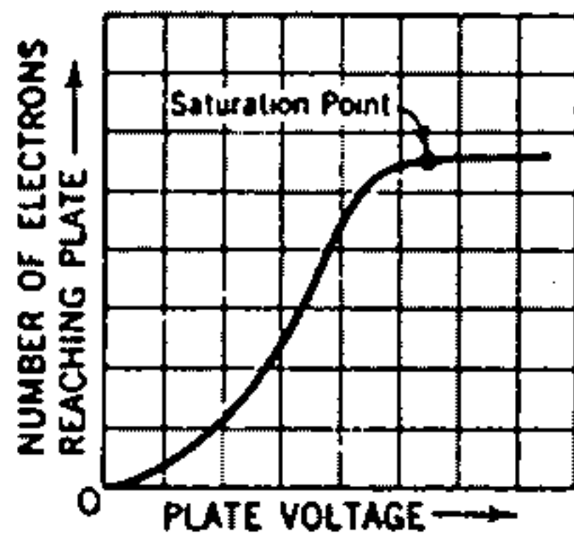
Fig. 5—Current characteristic of diode tube.
