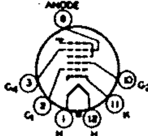
12AD ANODE = G 3 + G 4 + C FOCUSING ELECTRODE = G 4
