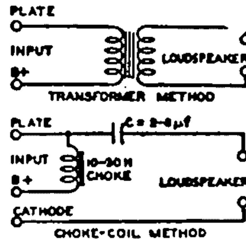
Fig. 123—Typical output-coupling devices.
