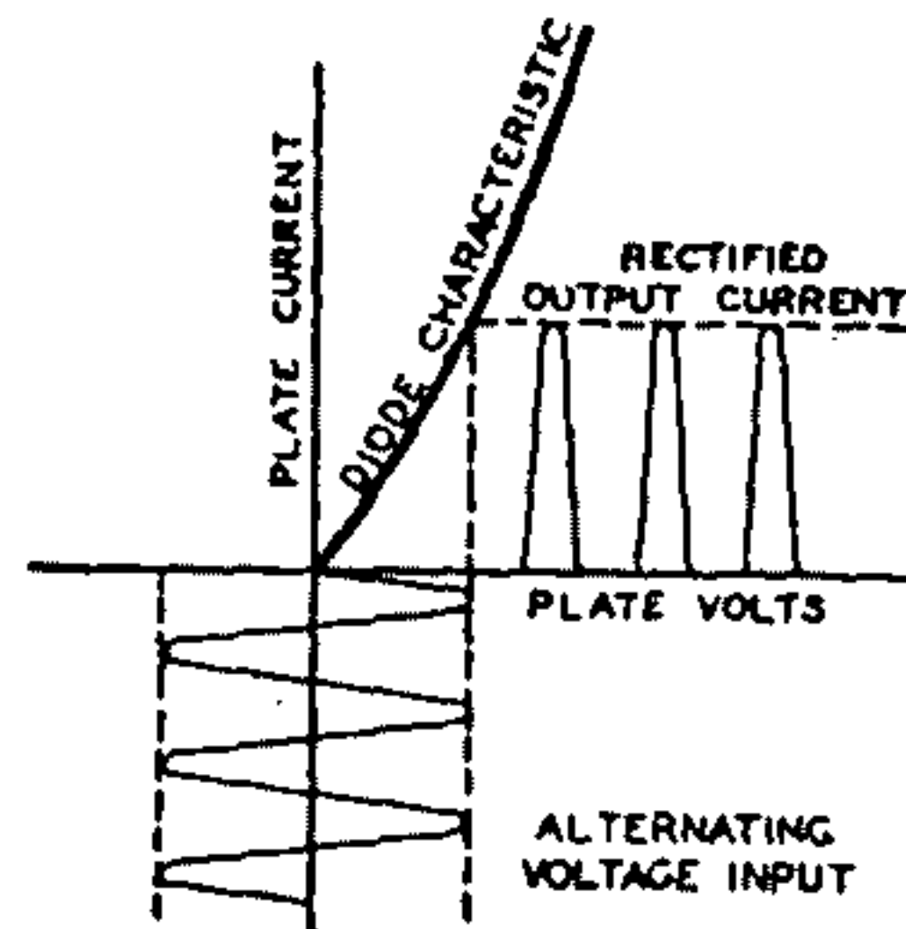
Fig. 4—Current characteristics of rectifier circuit.
