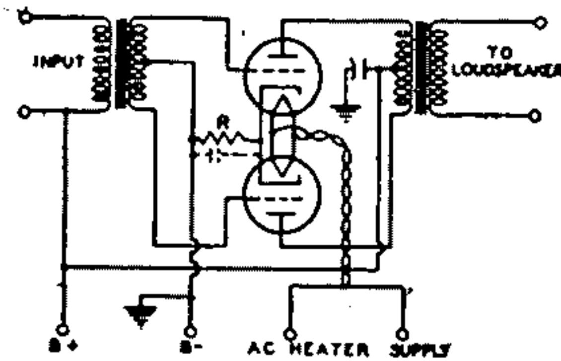
Fig. 40—Power amplifier with tubes connected in push-pull.
