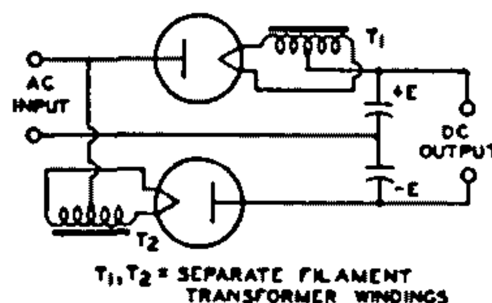
Fig. 19—Full-wave voltage-doubler circuit.
