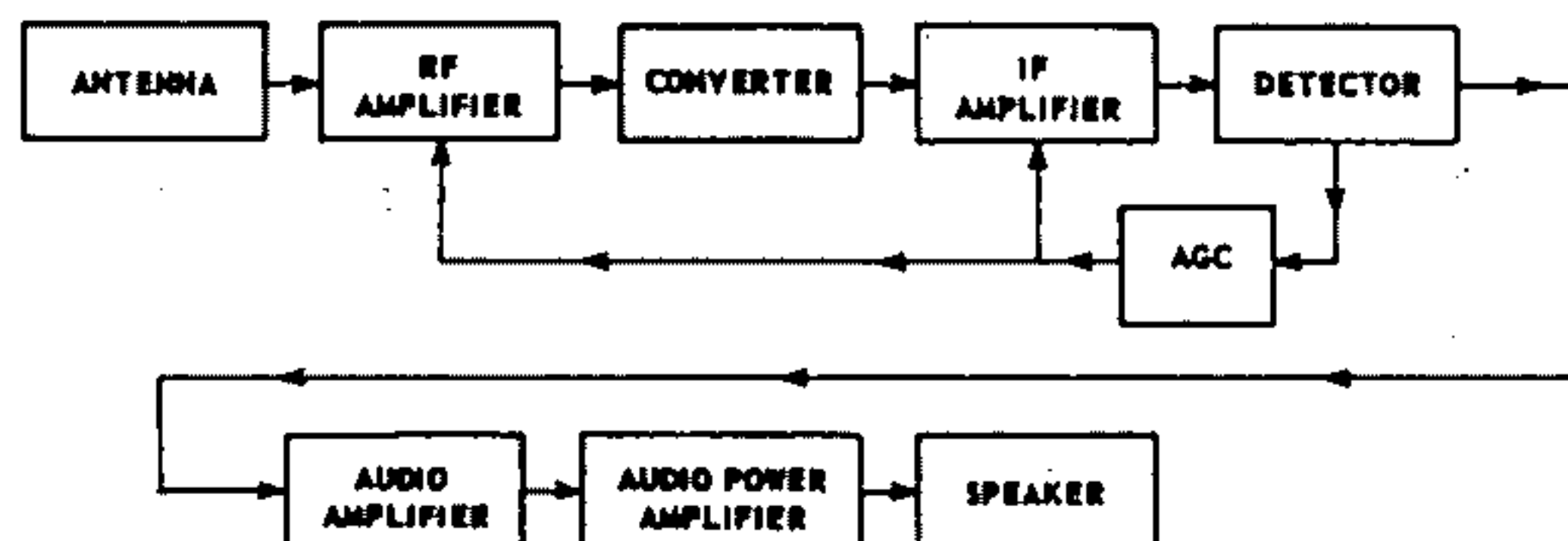
Fig. 14—Simplified block diagram for a broadcast-band receiver.
