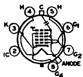
8KP ANODE = G_3 + G_4 + C_1 FOCUSING ELECTRODE = G_4
