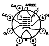
8HR ANODE = G_3 + G_4 + C_1 FOCUSING ELECTRODE = G_4
