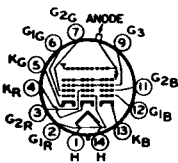
14AM ANODE = G 4 + G 5 + Cl + R FOCUSING ELECTRODE - G 3
