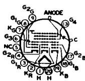
20A ANODE = G 3 + G 4 + Cl FOCUSING ELECTRODE - G 3
