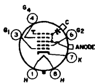
8KW ANODE = G_3 + G_4 + C_1 FOCUSING ELECTRODE = G_4
