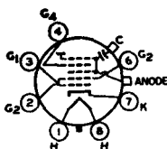
8JK ANODE = G_3 + G_4 + C_1 FOCUSING ELECTRODE = G_4
