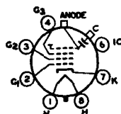
8JR ANODE = G_4 + C_1 FOCUSING ELECTRODE = G_3
