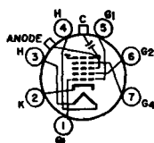
7GR ANODE = G_3 + G_4 + C_1 FOCUSING ELECTRODE = G_4
