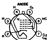
77G ANODE = G_3 + G_4 + C_1 AUTOMATIC FOCUSING
