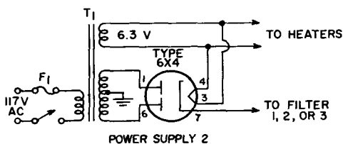
POWER SUPPLY 2
