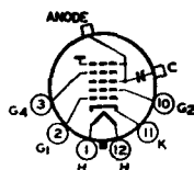
12AB ANODE = G_3 + G_4 + C_1 FOCUSING ELECTRODE = G_4
