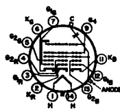
148H ANODE = G 3 + G 5 + Cl FOCUSING ELECTRODE - G 4
