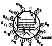
14B ANODE = G 3 + G 4 + Cl FOCUSING ELECTRODE - G 3
