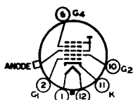
12M ANODE = G 3 + G 5 + Cl FOCUSING ELECTRODE - G 4
