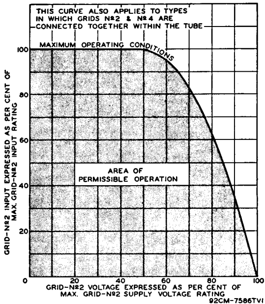
Fig. 128—Grid-No. 2 input rating curve.
