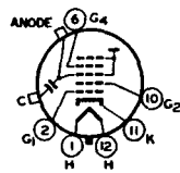
12L ANODE = G_3 + G_4 + C_1 FOCUSING ELECTRODE = G_4
