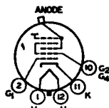
12S ANODE = G 3 + G 5 + Cl AUTOMATIC FOCUSING
