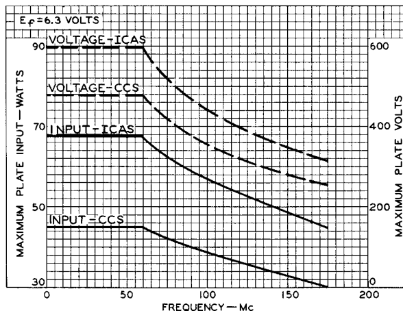
Rating Chart I for Type 7212 in Class C Telephony Service.
