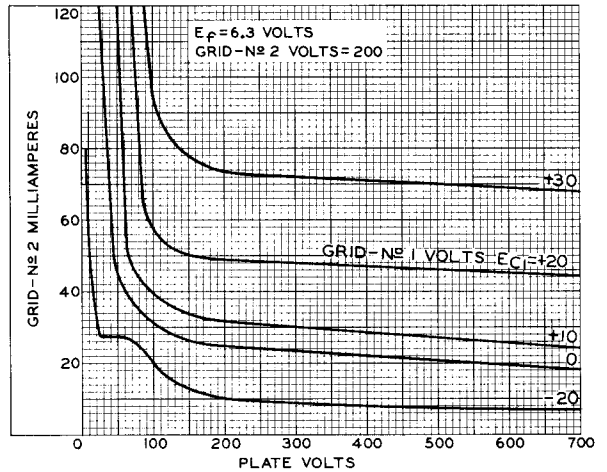
Fig. 6 - Average Characteristics of Type 7212.
