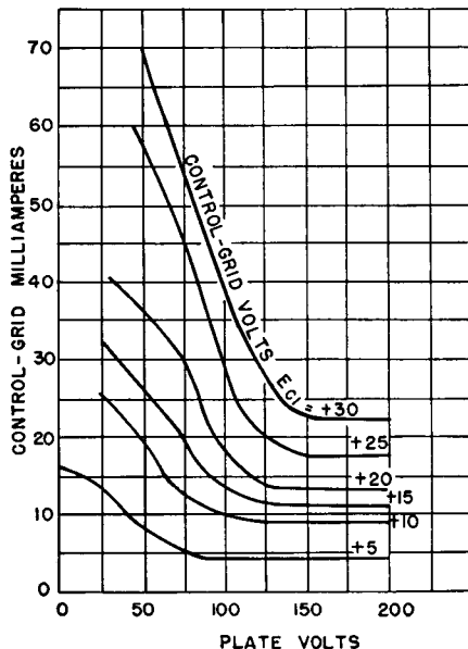
GL-807 TYPICAL CHARACTERISTICS (E r = 6.3 VOLTS, SCREEN VOLTS = 300)
