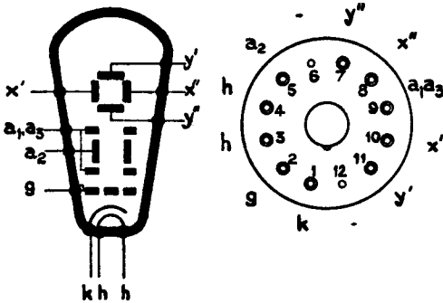
12-CONTACT PIN BASE
