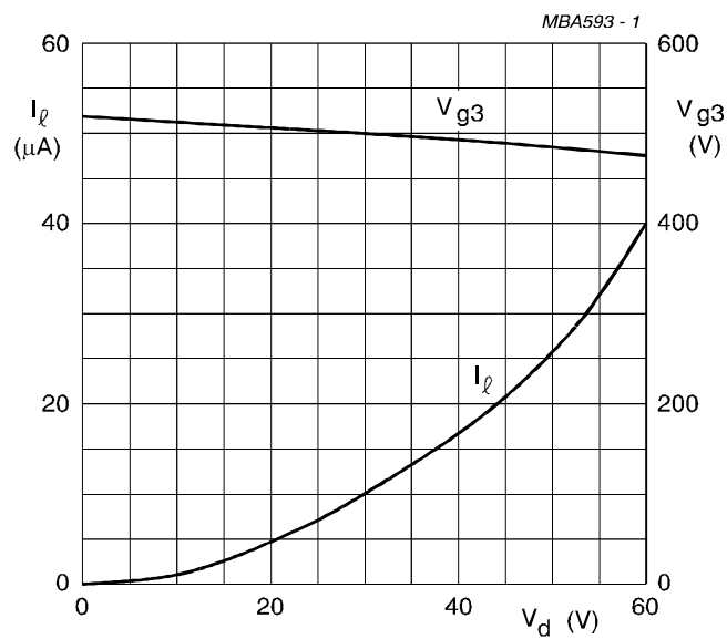
Fig.5 Screen current( I_l ) and focusing voltage ( V_{g3} ) as a function of grid drive voltage ( V_d ) at V_{g7} = 16 kV, V_{g5} = 2 kV; typical curves.
