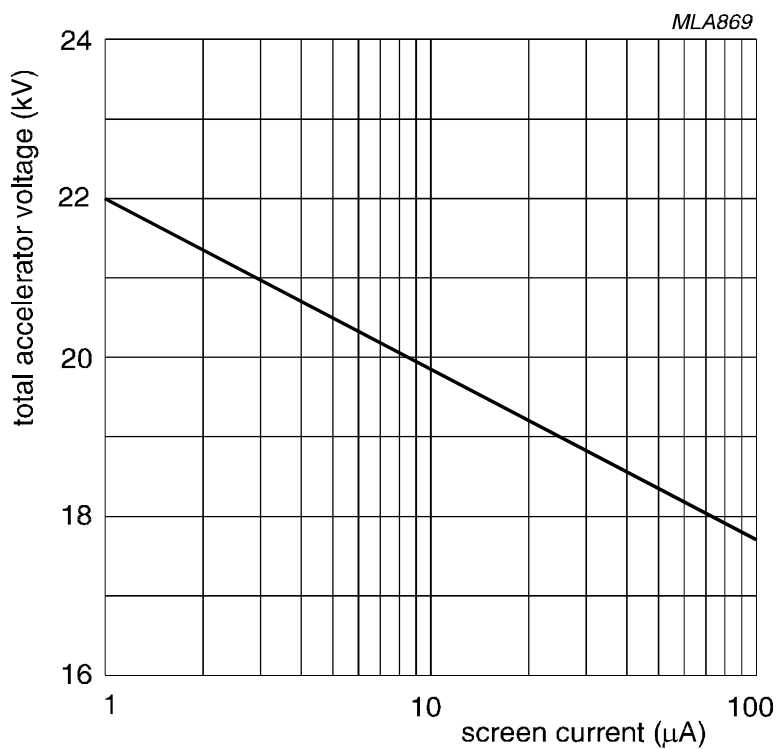
Fig. 6 0.5 mR/h isoexposure-rate limit curve. Measured according to EIA standard RS-502 , March 1989 (formerly TEPAC 104).
