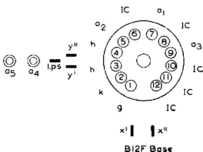
B12F Base
